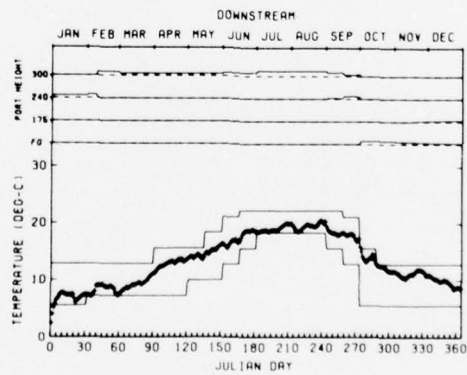
MARYSVILLE LAKE COMPUTED TEMPERATURES AT THE RELEASE, AFTERBAY, AND DOWNSTREAM INITIAL SIMULATIONS 100% ENTRAINMENT BY PUMPBACK 1962
