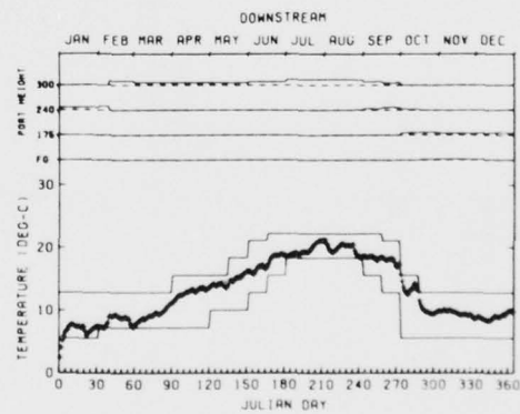
MARYSVILLE LAKE COMPUTED TEMPERATURES AT THE RELEASE, AFTERBAY, AND DOWNSTREAM INITIAL SIMULATIONS NO ENTRAINMENT BY PUMPBACK 1962
