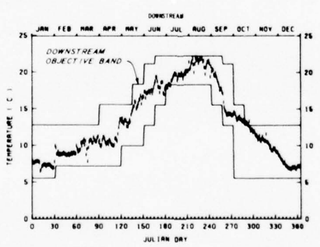
MARYSVILLE LAKE COMPUTED TEMPERATURES AT THE RELEASE, AFTERBAY, AND DOWNSTREAM FINAL SIMULATIONS PUMPBACK AT BOTTOM 1942 HYDROLOGY 1963 METEOROLOGY
