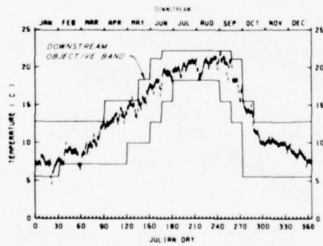
MARYSVILLE LAKE COMPUTED TEMPERATURES AT THE RELEASE, AFTERBAY, AND DOWNSTREAM FINAL SIMULATIONS PUMPBACK AT BOTTOM 1962 HYDROLOGY 1962 METEOROLOGY
