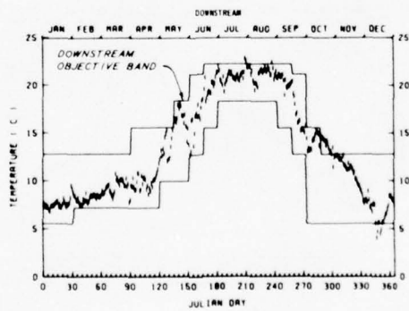
MARYSVILLE LAKE COMPUTED TEMPERATURES AT THE RELEASE, AFTERBAY, AND DOWNSTREAM FINAL SIMULATIONS NO PUMPBACK 1934 HYDROLOGY 1967 METEOROLOGY
