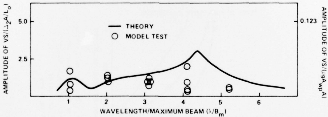
Figure 19 - Amplitude of Vertical Shear Force of SWATH 1 in Regular Beam Waves
