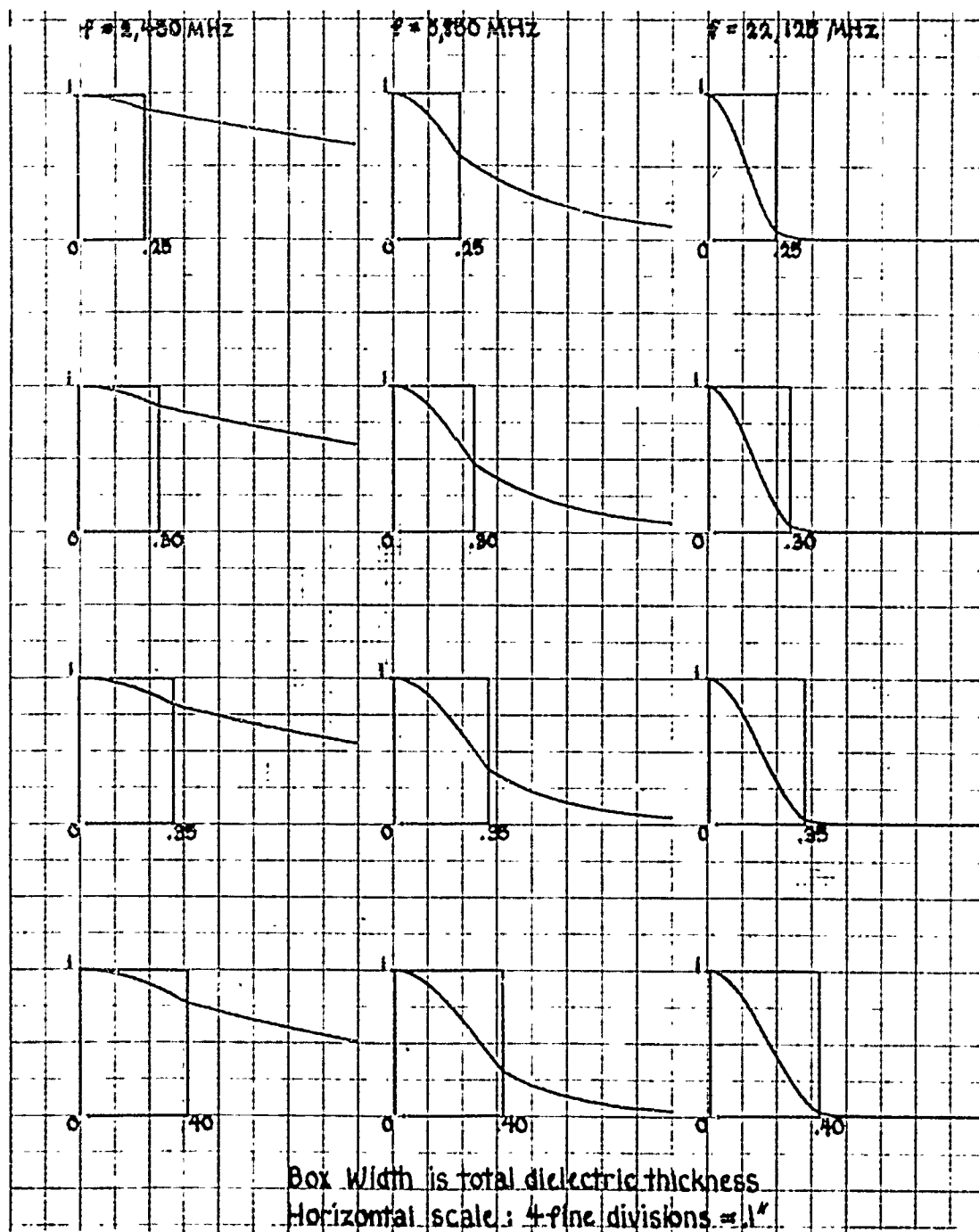
Figure F-2. Normalized power density (y-coordinate) versus vertical position (x-coordinate) for TM even mode, \epsilon_1 = 2.0 , \epsilon_2 = 1.0
