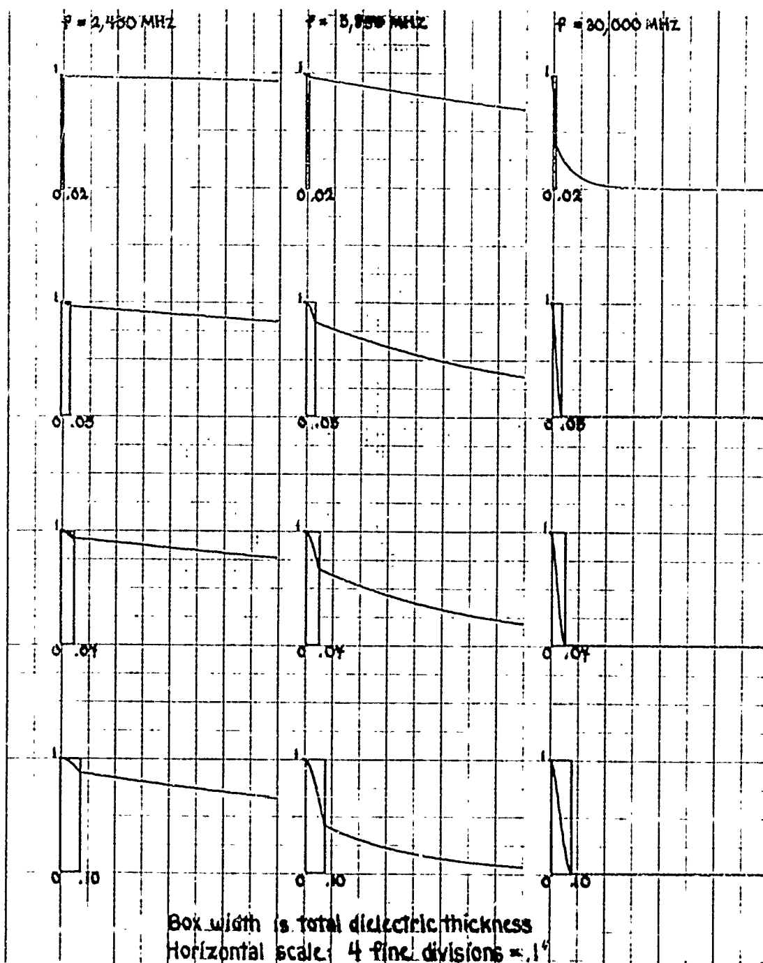
Figure F-20. Normalized power density (y-coordinate) versus vertical position (x-coordinate) for T11 even mode, \epsilon_1 = 9.0 , \epsilon_2 = 1.0
