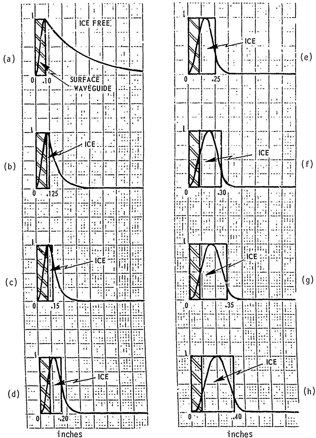
Figure 3. Calculated power density versus ice accretion on a dielectric surface waveguide, TE_1 mode ( f = 22,125 MHz)
