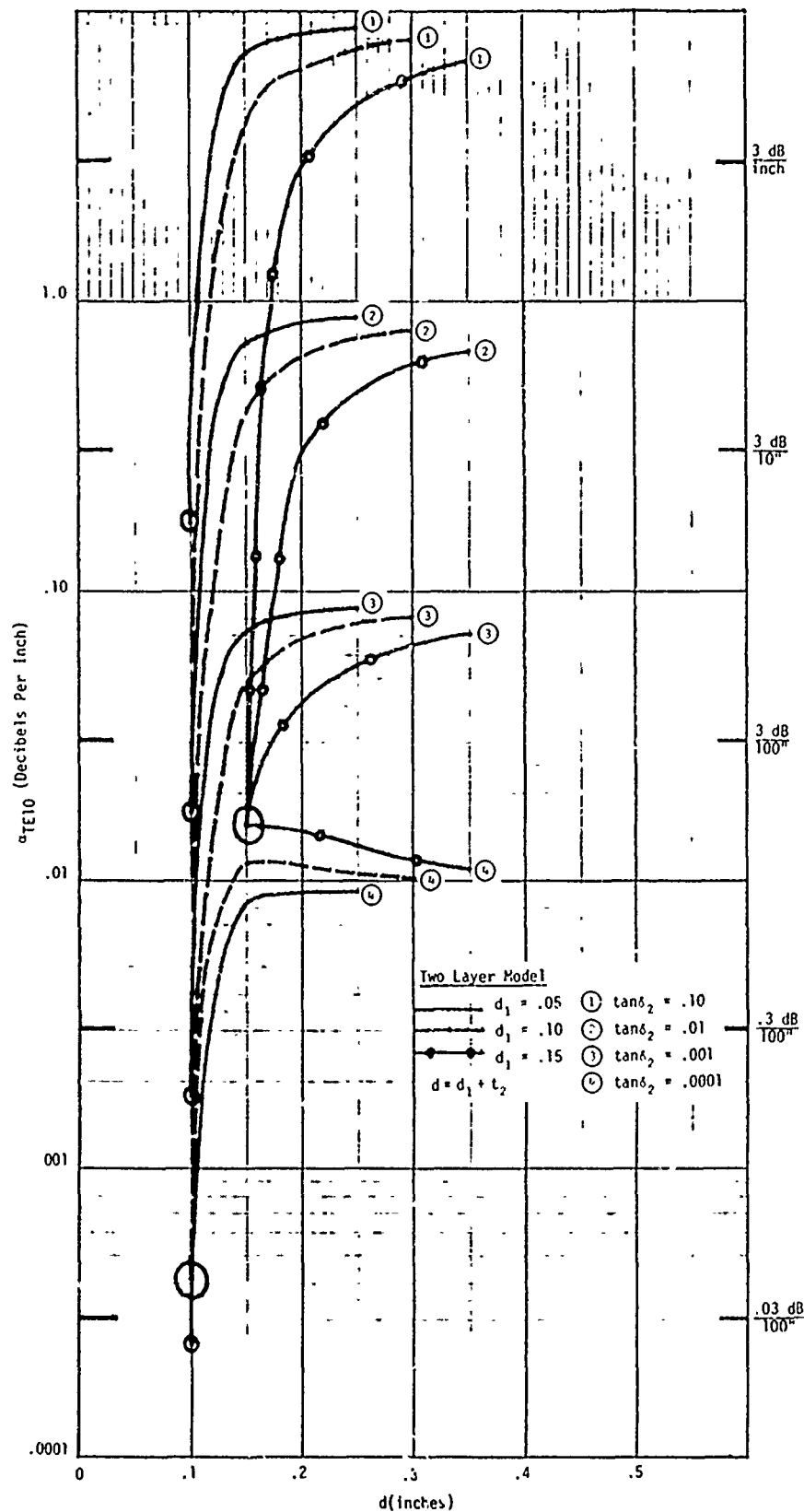
Figure 30. Attenuation versus thickness of dielectric for TE odd mode f = 22,125 MHz, \epsilon_1 = 2.8 , \tan \delta_1 = .0002 , \epsilon_2 = 1.0
