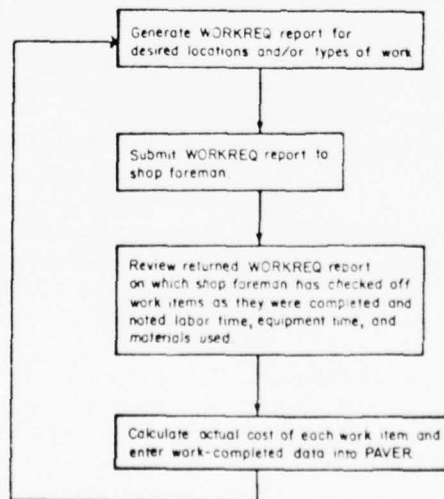
Figure 28. Using PAVER for assigning M&R work.
