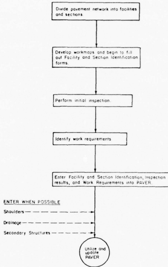
Figure 27. Initiating the PAVER data base.
