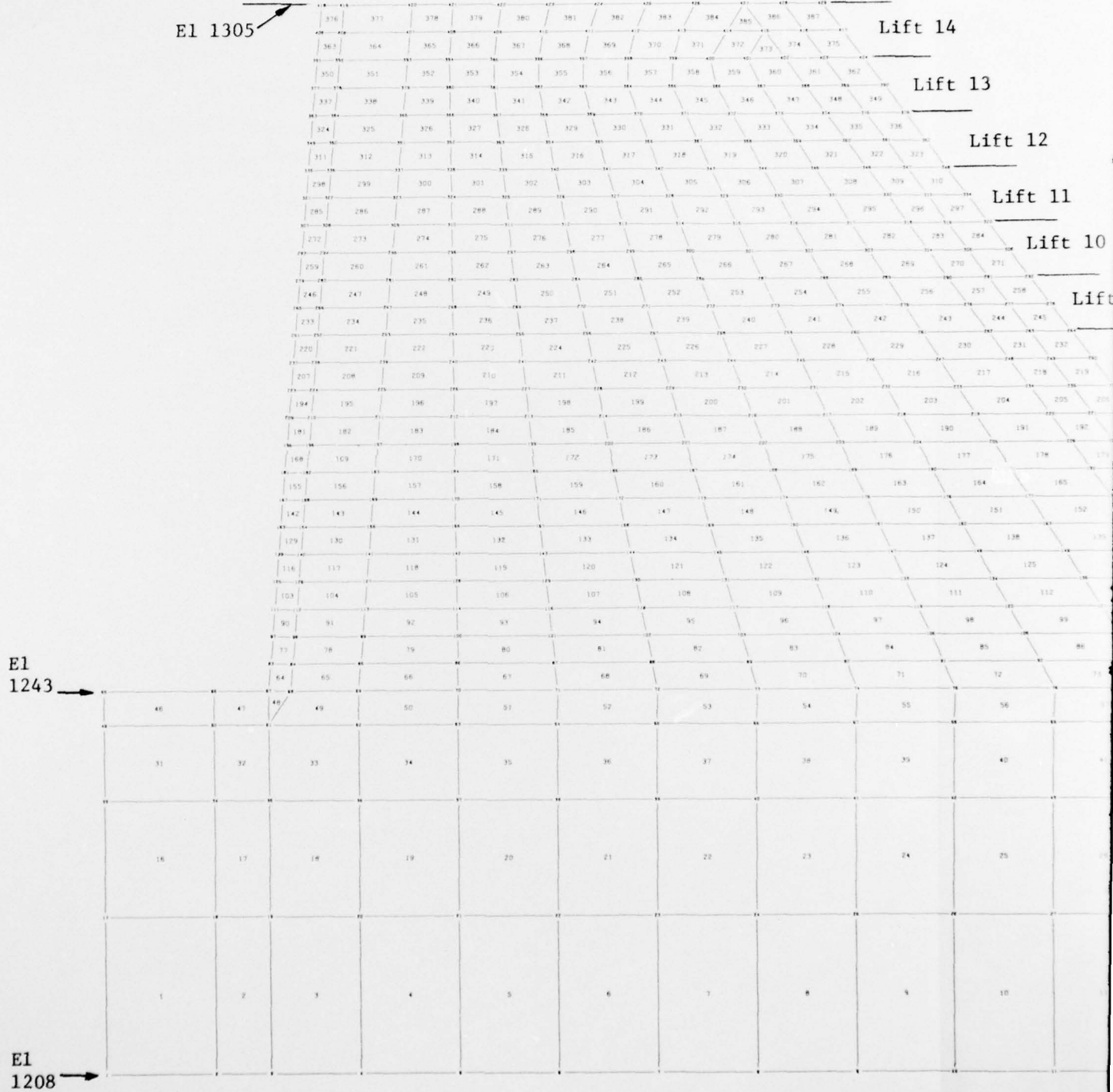
Figure 1. Finite element model
