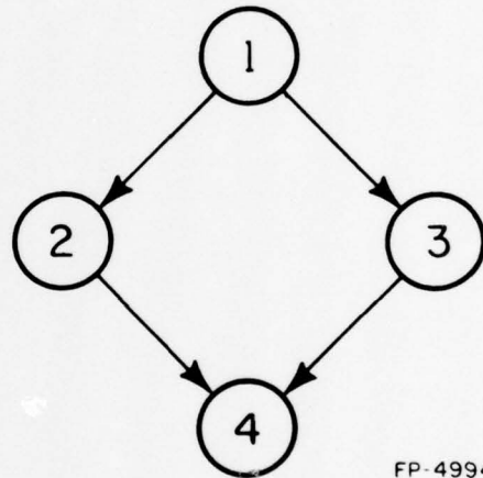
Fig 2.2b Directed Graph
