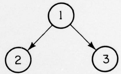
Fig 2.3 Example Blocks
