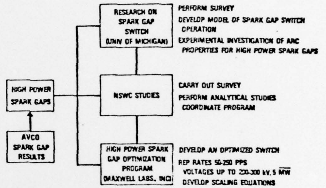
FIGURE 2. PROGRAM OUTLINE
