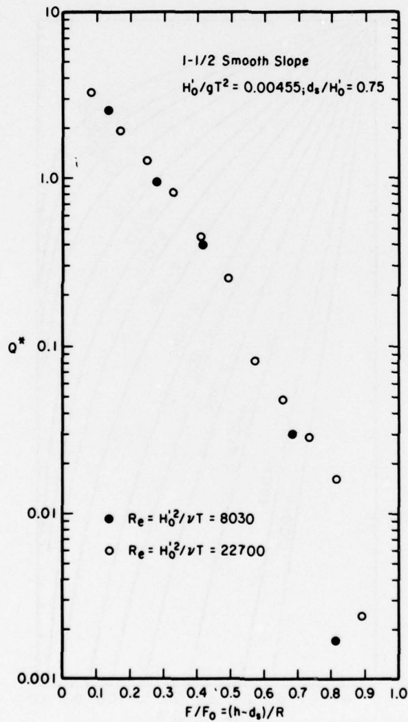
Figure 2. Typical data plot, 1 on 1 1/2 smooth slope, H_0'/gT^2 = 0.00455 ; d/H_0' = 0.75 .
