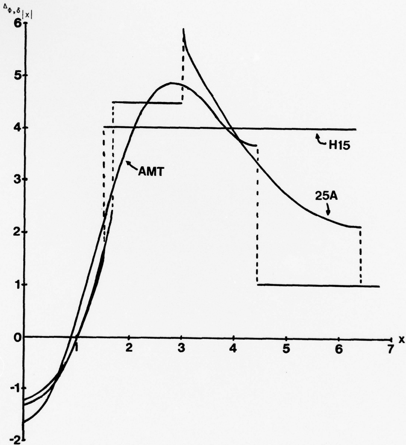
B. \Delta_{\phi, \delta}|x| for H15, 25A, and AMT
