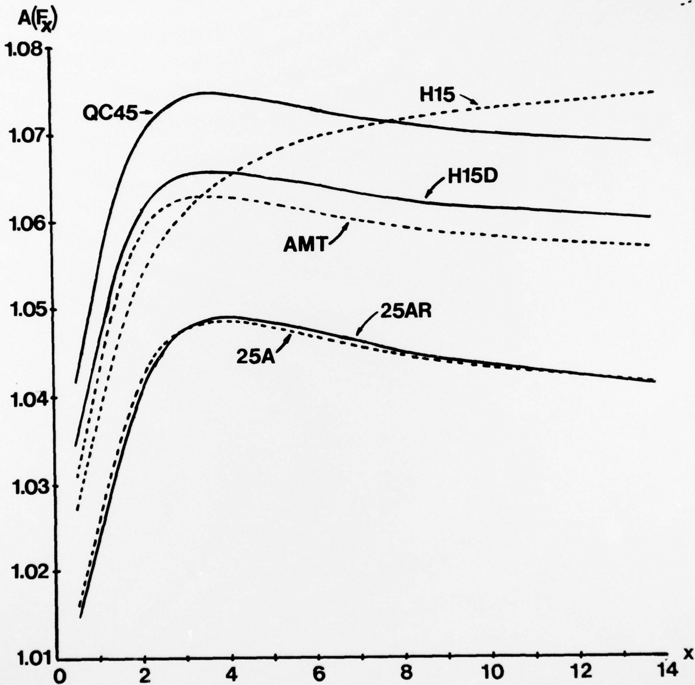
G. Asymptotic Variances of H15, 25A, AMT, H15D, 25AR, and QC45 at F_x = .99\phi + .01N_x
