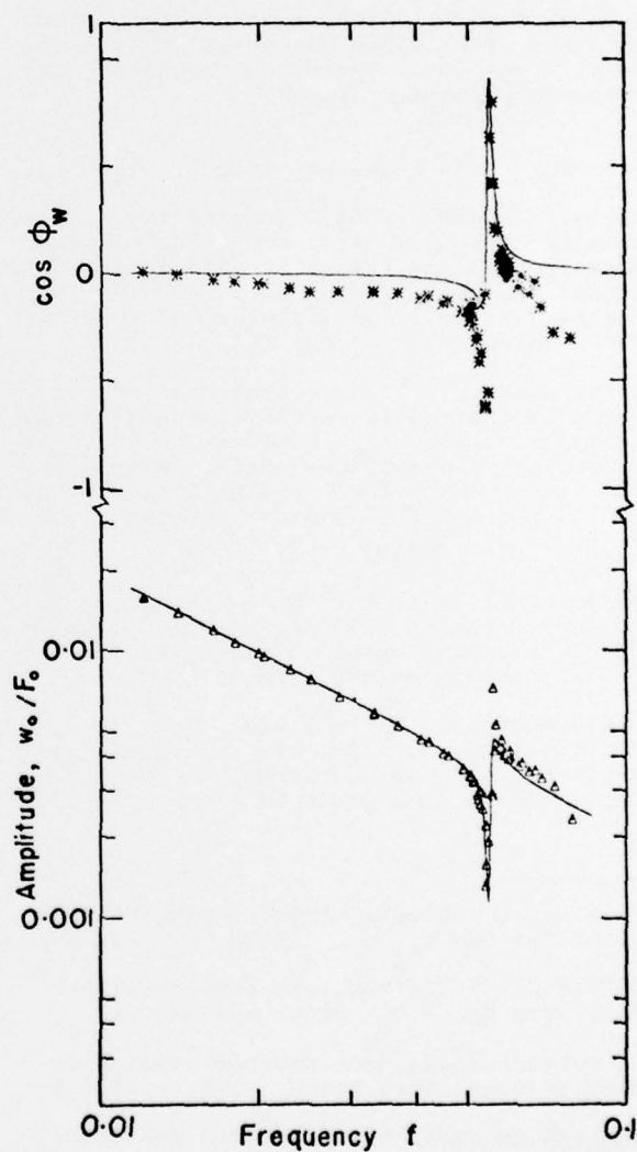
Figure 5 Heave Transfer Function 5-Caliber Model, Flow On
