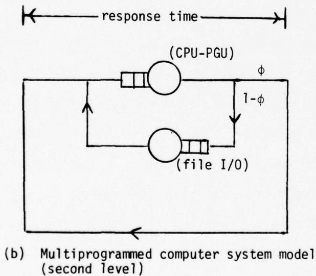
Fig. 8.1: Hierarchical Models of a Multiprogrammed Computer System
