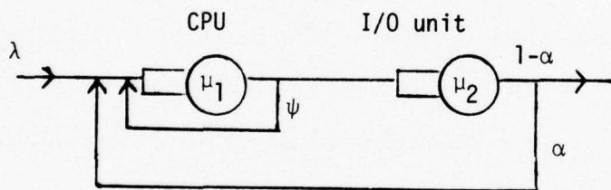
(a) open queueing network model
