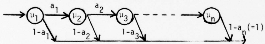
Fig 3.1 Representation of service time distributions by the method of stages
