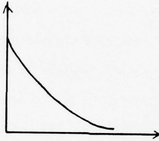
(a) density function dF_w(t)/dt
