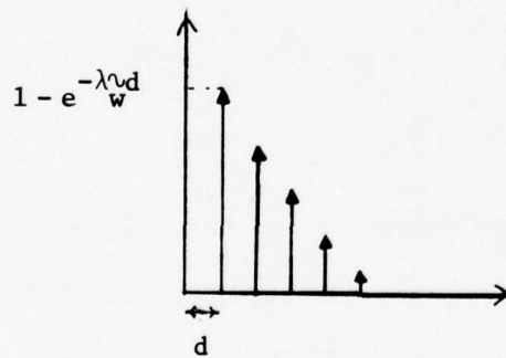
(b) discrete approximation P_{F_w}(k)
