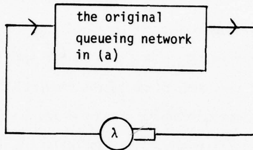
(b) approximate closed queueing network model
