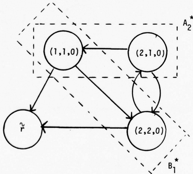
Fig. 5.6: State transition diagram of Z^*(t) and subsets A_2^* and B_1^* for passage time T^*
