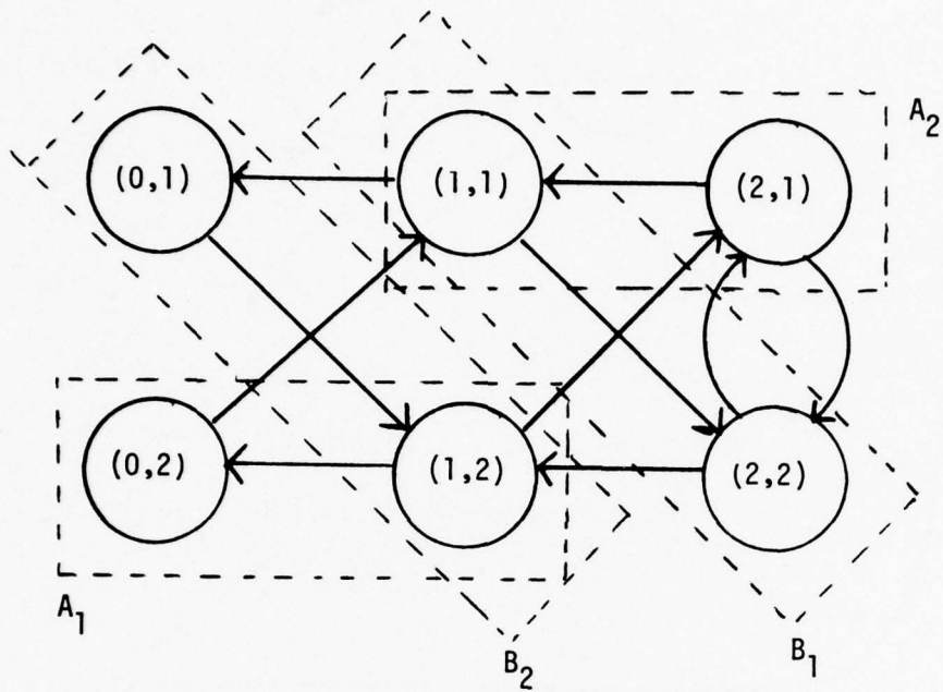
Fig. 5.5: State transition diagram of Z(t) = (Q_0(t), K(t)) and subsets A_i and B_i for passage time T^*
