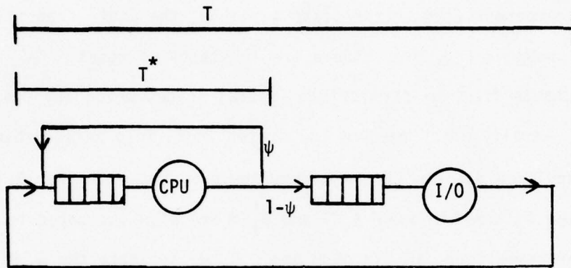
Fig. 5.1: A Closed Two Server Queueing Model
