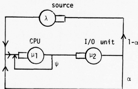
(b) approximate closed queueing network model
