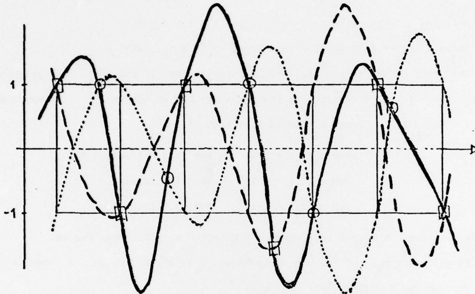
Figure 1. Schematic drawing of F_i (solid), F_j (dashed) and -F_j (dotted) for n = 6 , i = 3 , j = 5 . The graphs of F_i and (-1)^{j-i}F_j cross at the n points indicated by \square , those of F_i and -(-1)^{j-i}F_j cross at the n - 1 points indicated by \circ .
