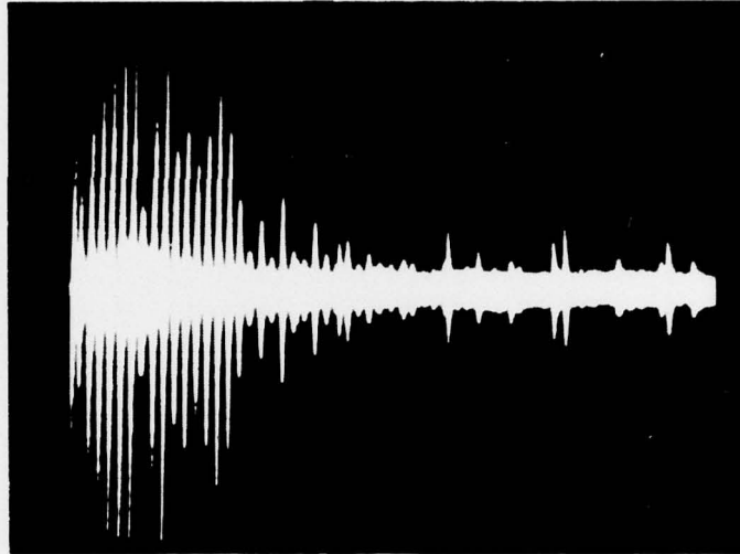
Figure 6c. Typical acoustic return from pilot study. Freq. = 680.3 kHz; Sweep = 5 msec/div. Amp. = 0.02 V/div.; Temp. = -0.3°C. Arrow indicates approx. 125-ft folded path length.
