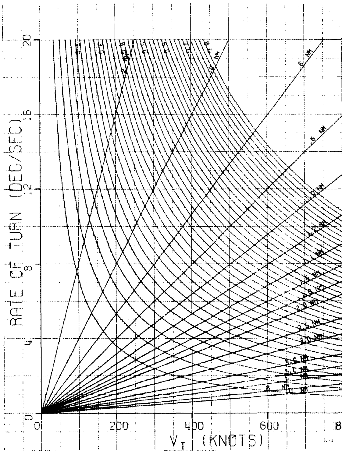
RATE OF TURN vs V_{TRUE}
