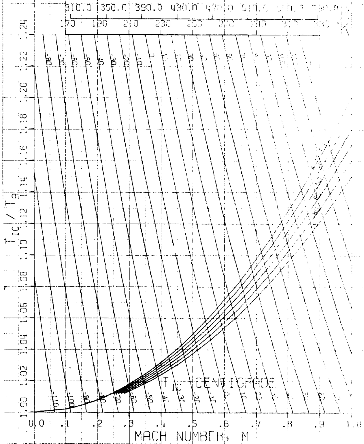
T_{IC}/T_A vs MACH
