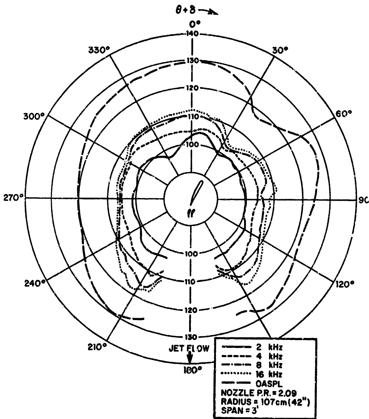
FIG. 78. POLAR PLOT OF ACOUSTIC FAR FIELD OF AUGMENTER WING OF FIGURE 75 [85].
