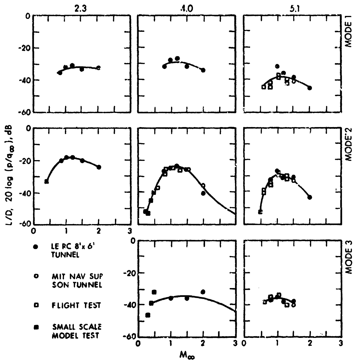
FIG. 115. MACH NUMBER DEPENDENCES OF RESONANT MODE LEVELS IN LEADING-EDGE AREAS OF CAVITIES [126].
