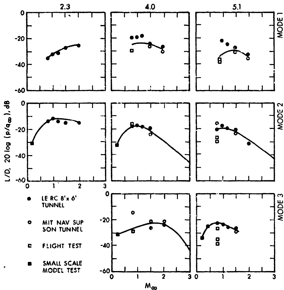
FIG. 116. MACH NUMBER DEPENDENCES OF RESONANT MODE LEVELS IN TRAILING-EDGE AREAS OF CAVITIES [126].
