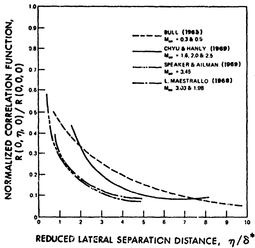
FIG. 89. NORMALIZED LATERAL BROAD BAND SPACE-TIME CORRELATION FOR ATTACHED TURBULENT FLOW [106].
