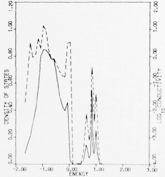
FIG. 11. Then dc conductivity (dashed line) of a three-dimensional alloy with V_1 = +0.75 and c = 0.1 . Density of states taken from Fig. 7 is shown in the solid line. Energy is in units of half-bandwidth.
