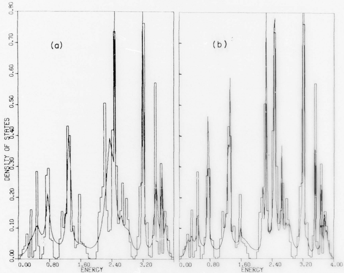
FIG. 5. (a) Density of states for a (50-50) concentration one-dimensional alloy with V_A = 2.0 , V_B = -2.0 . Histogram is exact calculations from Ref. 4. The full band is obtained by reflecting the portion shown through the origin. These results were computed from \text{Im}\Sigma = -0.80 and \text{Re}\Sigma obtained from \text{Im}\Sigma by Eq. (8), including the exact scattering from all configurations of a central atom and its four nearest neighbors. (b) Extension of the above results to a cluster of seven atoms using the same \Sigma(x) . This result is comparable in accuracy and wealth of detail to the best self-consistent calculation to date, Ref. 4. Energy is in units of half-bandwidth.
