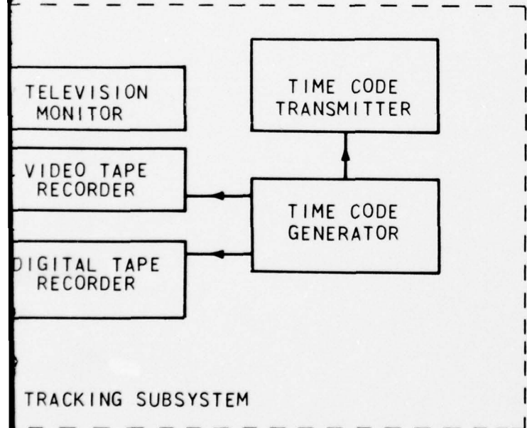
CATION NOISE MEASUREMENT SYSTEM BLOCK DIAGRAM
