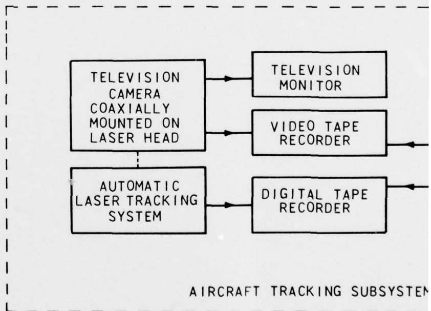
FIGURE 8.1 CERTIFICATION NOISE MEASUREMENT SYSTEMS
