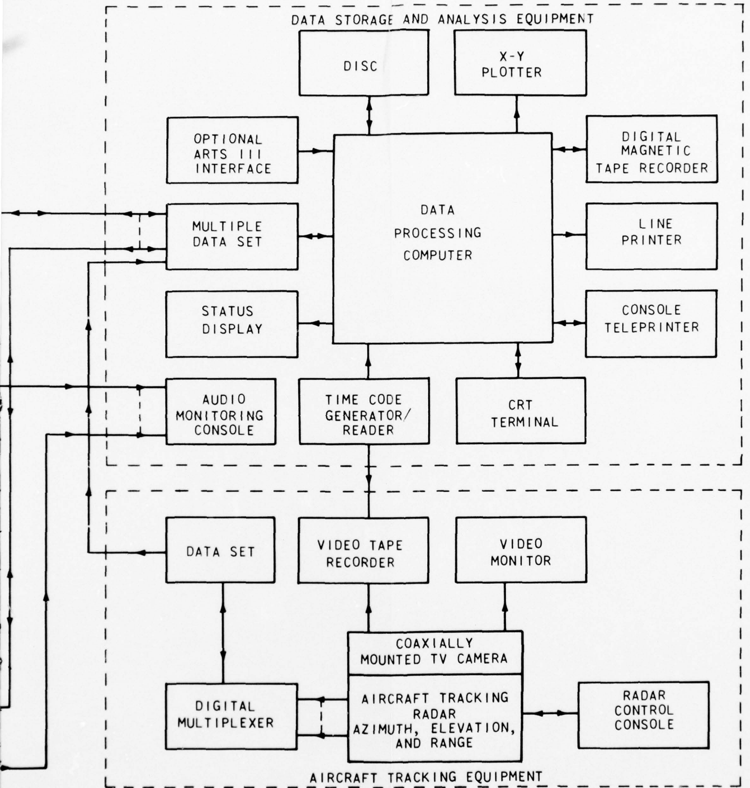
RESEARCH SYSTEM BLOCK DIAGRAM
