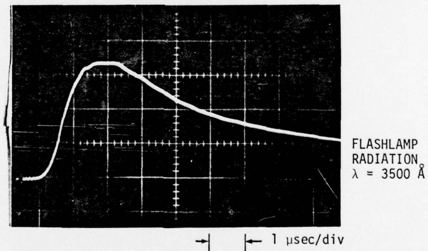
Figure 2. Oscilloscope traces of flashlamp current and light output at 3500 Å. The capacitor charge voltage was 10 kV, corresponding to an energy of 50 J/lamp. The current was measured with a Pearson probe and the flashlamp radiation was detected with a vacuum photodiode.
