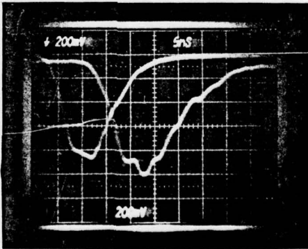
Figure 5. XeF fluorescence at 3533 \text{ \AA} for a He + 4% Xe + 0.13% \text{F}_2 gas mixture at total pressures of (a) 760 torr and (b) 500 torr. The photodiode response to the XeF laser emissions precedes the photomultiplier response to the fluorescence due to the transit time of the electrons in the photomultiplier.
