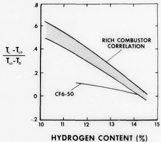
Figure 20.4.12 Effect of Lean Operation on Combustor Fuel Sensitivity
