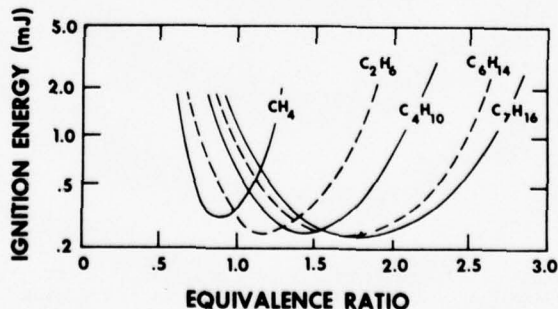
Figure 15.4.4 Minimum Ignition Energies
