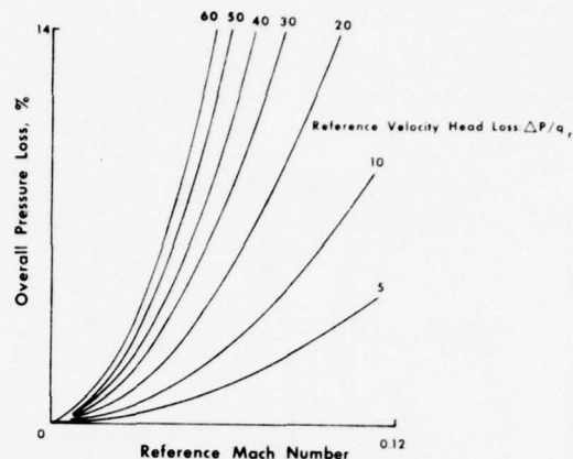
Figure 20.2.1 Pressure Loss Correlation
