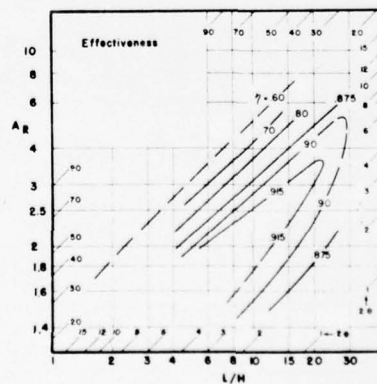
Figure 20.2.6 Diffuser Design and Performance Characteristics
