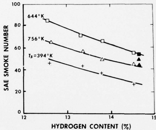
Figure 20.4.10 Smoke Emission Dependence on Hydrogen Content
