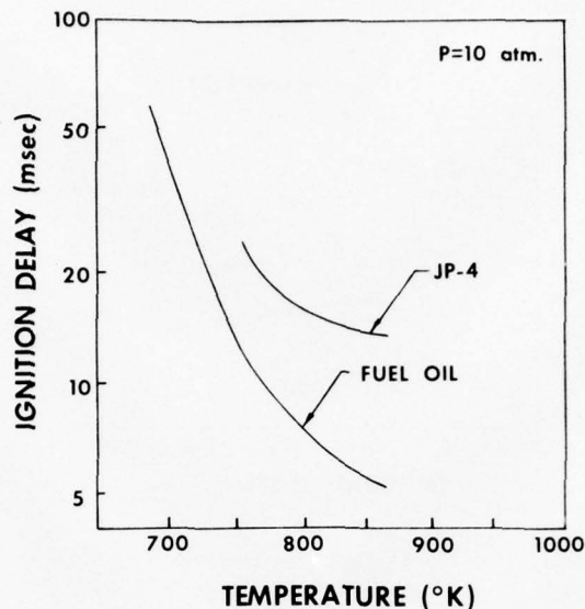
Figure 15.4.3 Ignition Delay Times for Practical Fuels.
