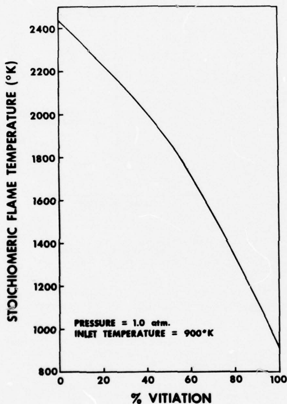
Figure 15.2.6 Effect of Vitiation on Stoichiometric Flame Temperature.
