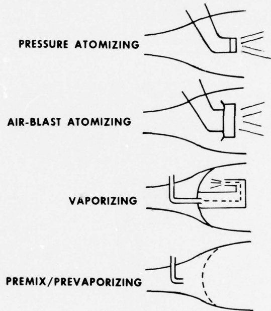
Figure 20.2.11 Fuel Injection Methods
