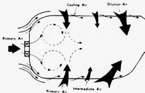
Figure 20.1.9 Main Combustor Airflow Distribution
