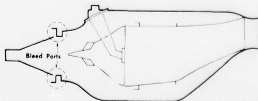
Figure 20.4.13 HMC with Advanced Bleed Diffuser
