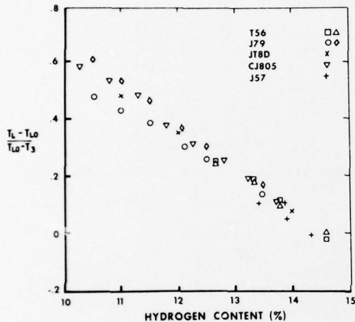
Figure 20.4.9 Liner Temperature Correlation for Many Combustor Types
