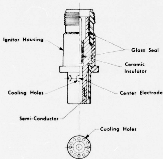
Figure 20.2.13 Spark Igniter
