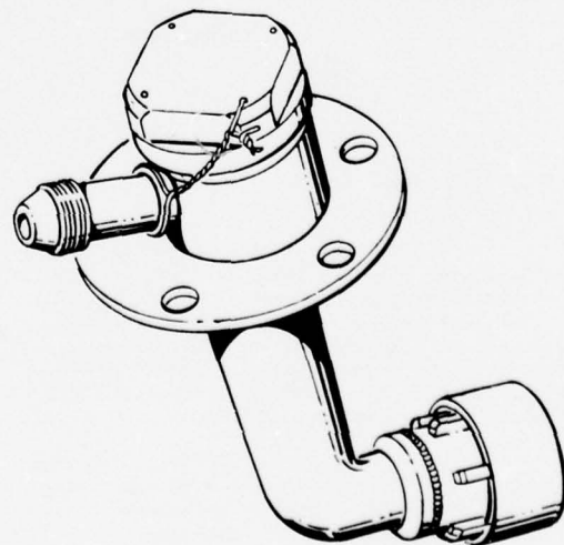
Figure 20.2.12 Pressure Atomizing Fuel Injector
