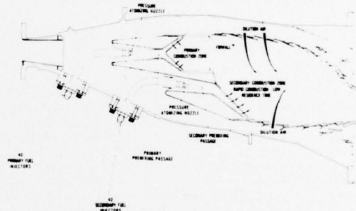
Figure 20.4.5 Staged Premix Combustor. JT9D Engine
