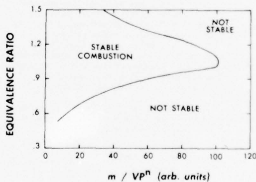
Figure 15.3.5 Stirred Reactor Stability Dependence on Equivalence Ratio.
