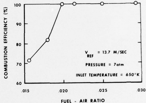
Figure 20.5.3 Catalytic Combustor Efficiency
