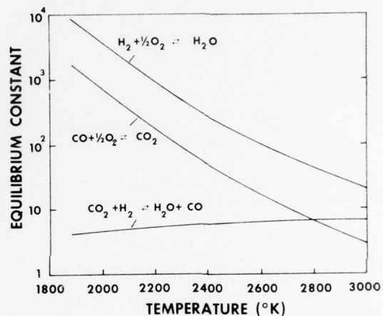
Figure 15.1.2 Equilibrium Constants for Important Dissociation Reactions.
