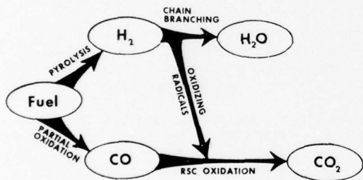
Figure 15.1.4 Hydrocarbon Combustion Chemistry Schematic.
