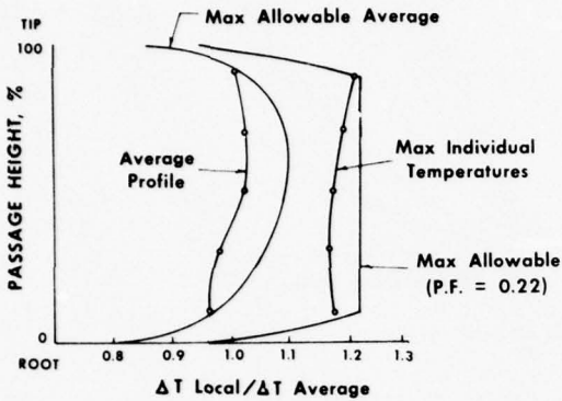
Figure 20.2.2 Radial Temperature Profile at Combustor Exit
