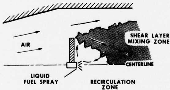
Figure 15.3.3: Simplified Representation of a Turbine Combustion System.
