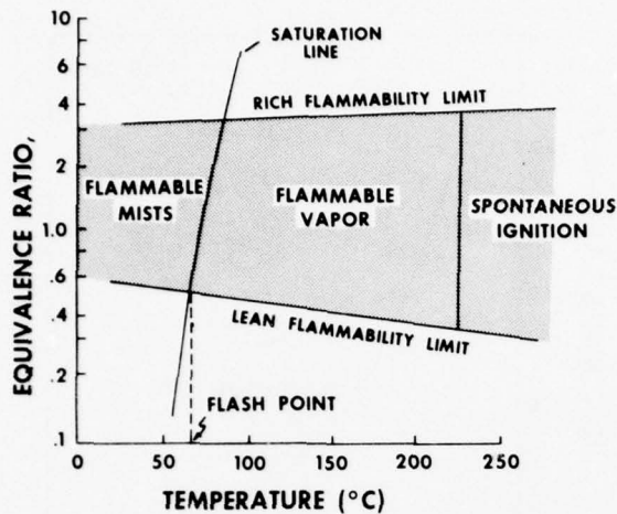
Figure 15.4.1: Flammability Characteristics for a Kerosene-Type Fuel in Air at Atmospheric Pressure.
