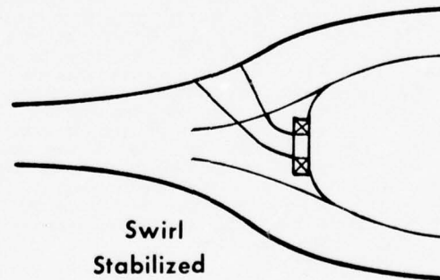
Figure 20.2.8 Combustor Dome Types
