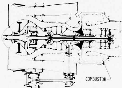
Figure 20.1.8 TFE 731 Turbofan Engine with Reverse-Flow Combustor
