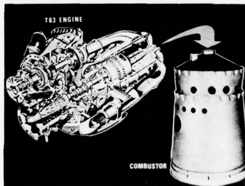
Figure 20.1.2 T63 Turboprop Engine With Can Combustor
