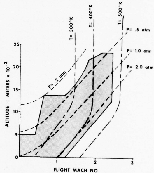
Figure 20.2.4 Ignition/Relight Envelope
