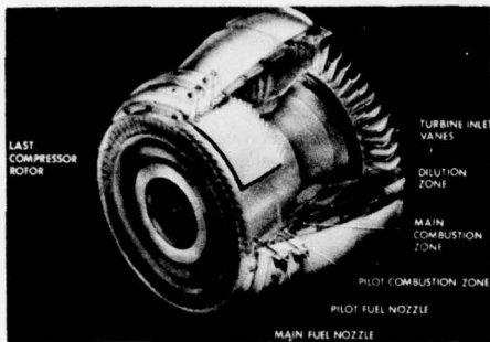
Figure 20.4.14 Swirl Burning HMC
