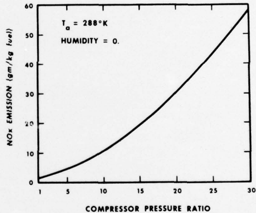
Figure 20.4.3 Dependence of Sea Level Standard Day \text{NO}_x Emissions on Compressor Pressure Ratio of Current Engines
