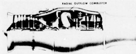
Figure 20.1.6 WR19 Turbofan Engine
