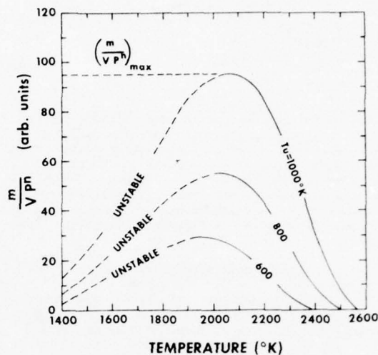
Figure 15.3.4 Perfectly Stirred Reactor Operating Conditions.
