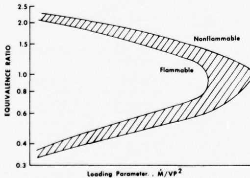
Figure 20.2.3 Combustion Stability Characteristics
