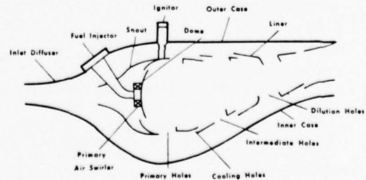
Figure 20.2.5 Component Identification
