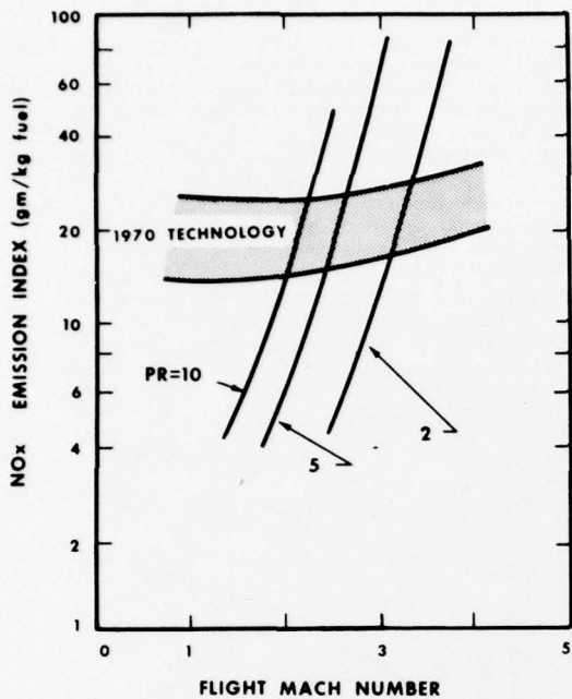
Figure 20.4.4 Dependence of \text{NO}_x Emission on Flight Mach Number
