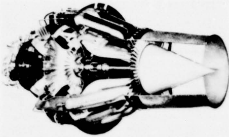
Figure 20.1.3 J33 Turbojet Engine With Can Combustors
