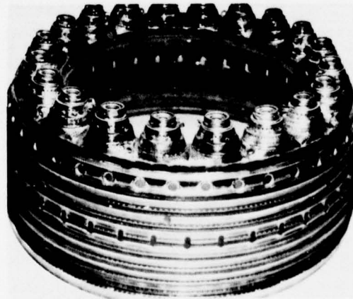
Figure 20.1.7 JT9D Annular Combustor
