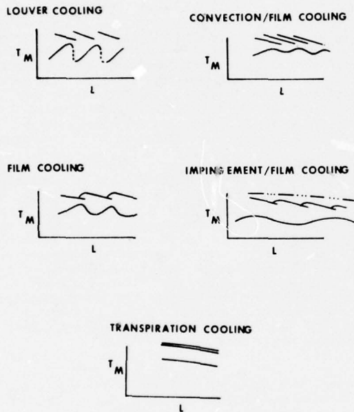
Figure 20.2.10 Liner Cooling Characteristics
