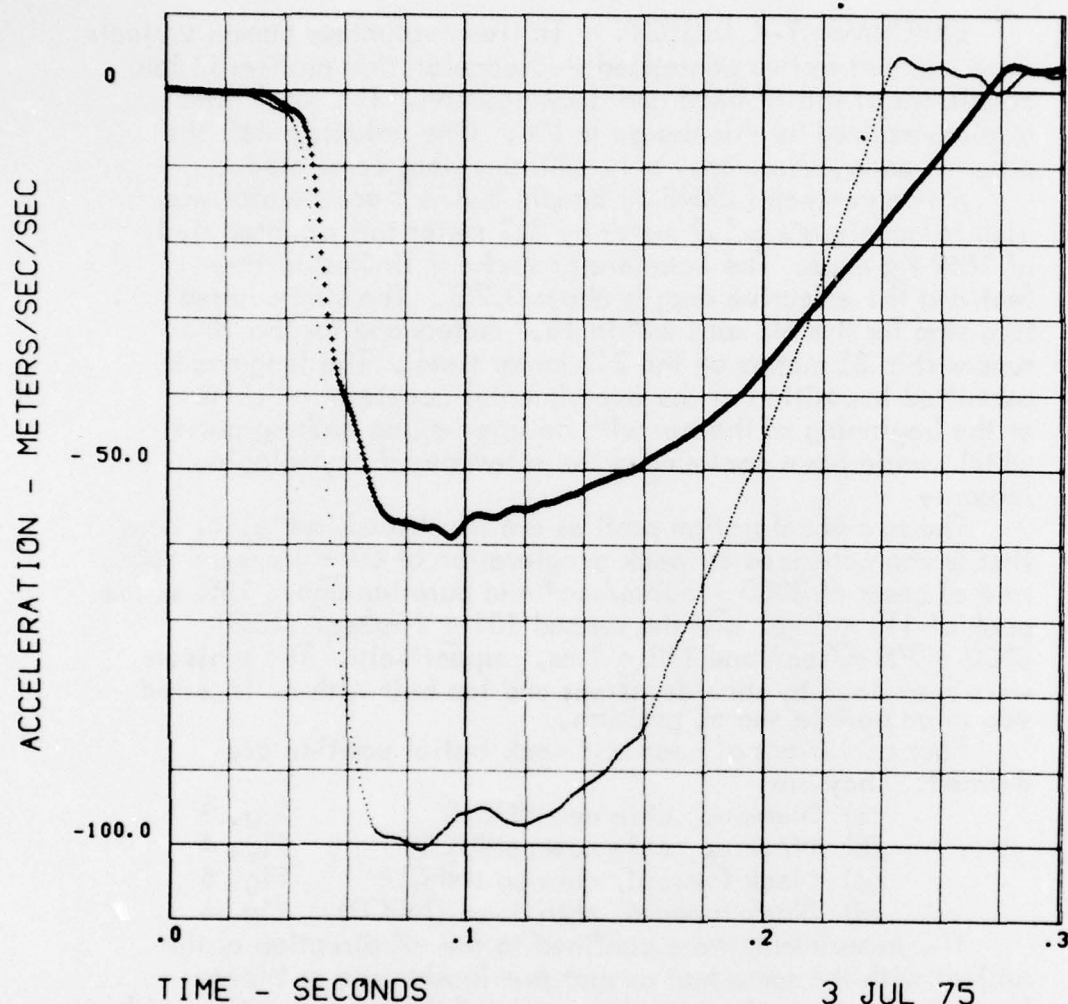
Fig. 2 - Typical sled acceleration profiles (6 and 10G)
