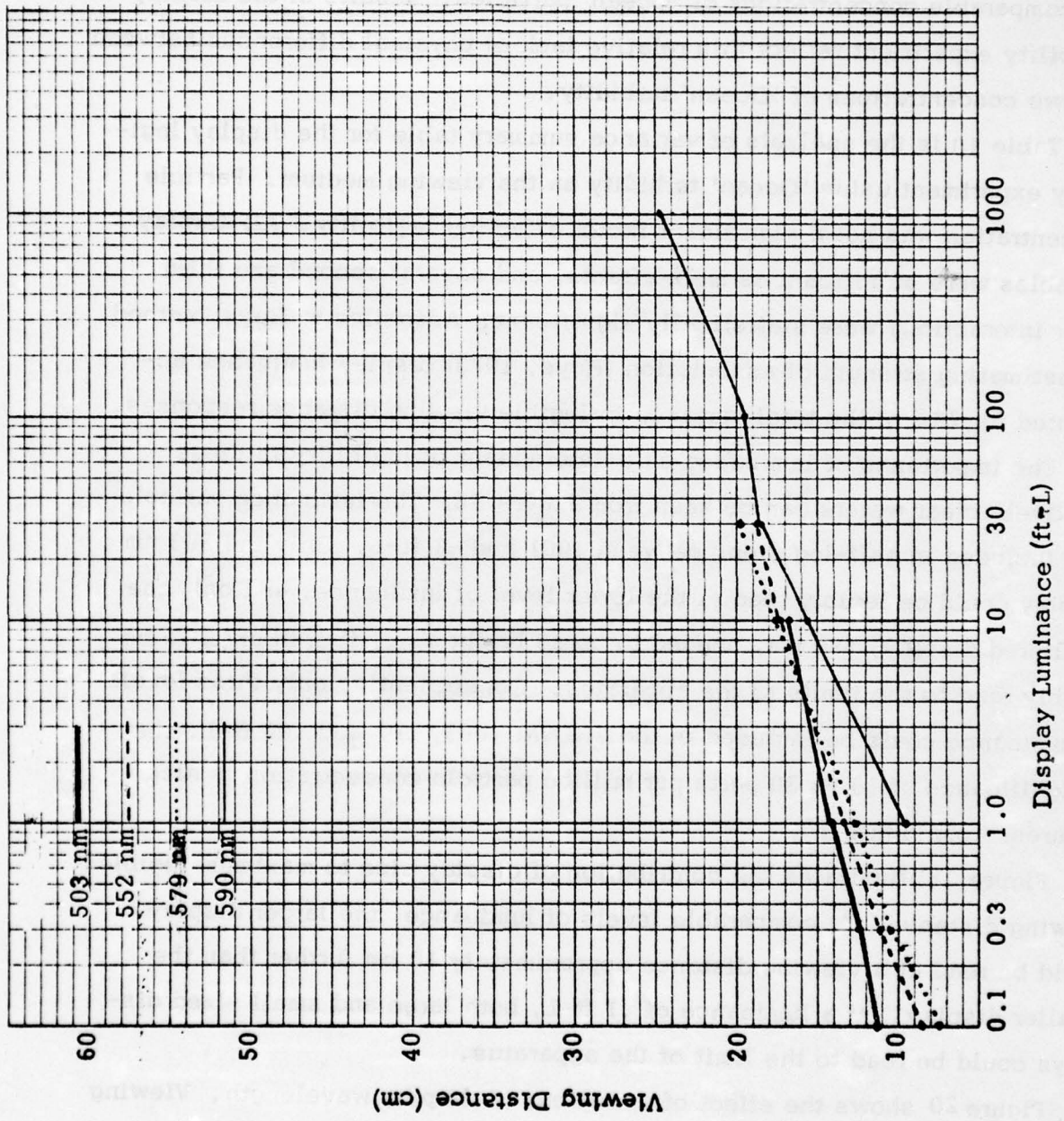
Figure 17. Maximum Legible Viewing Distance in Harbor-30 Turbidity as a Function of Display Wavelength.
