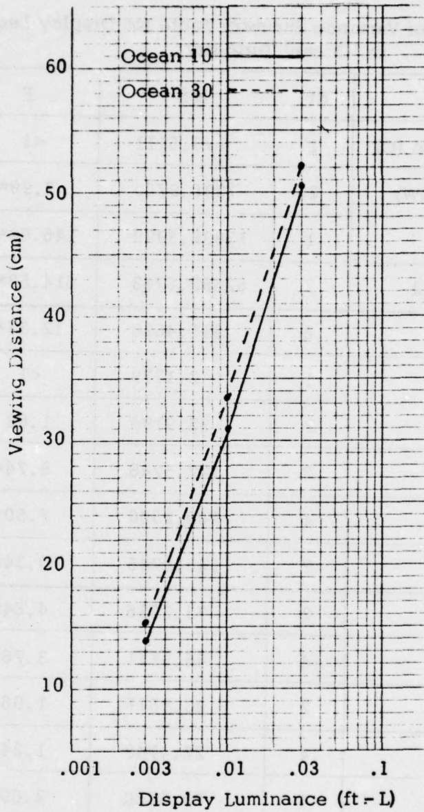
Figure 18. Maximum Legible Viewing Distance in Ocean Turbidity as a Function of Display Luminance
