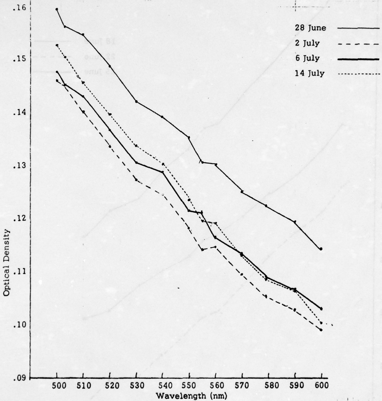
Figure 10. Optical Density vs Wavelength for Four Samples of Ocean-10 Turbidity
