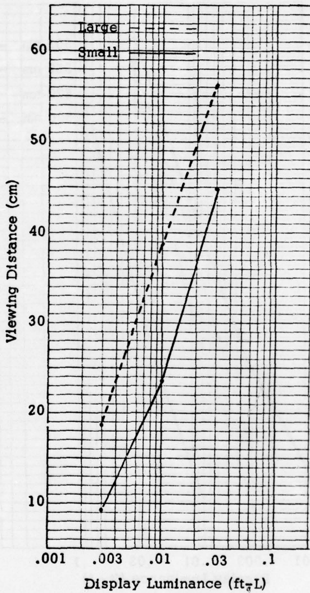
Figure 19. Maximum Legible Viewing Distance in Ocean Turbidity as a Function of Display Size
