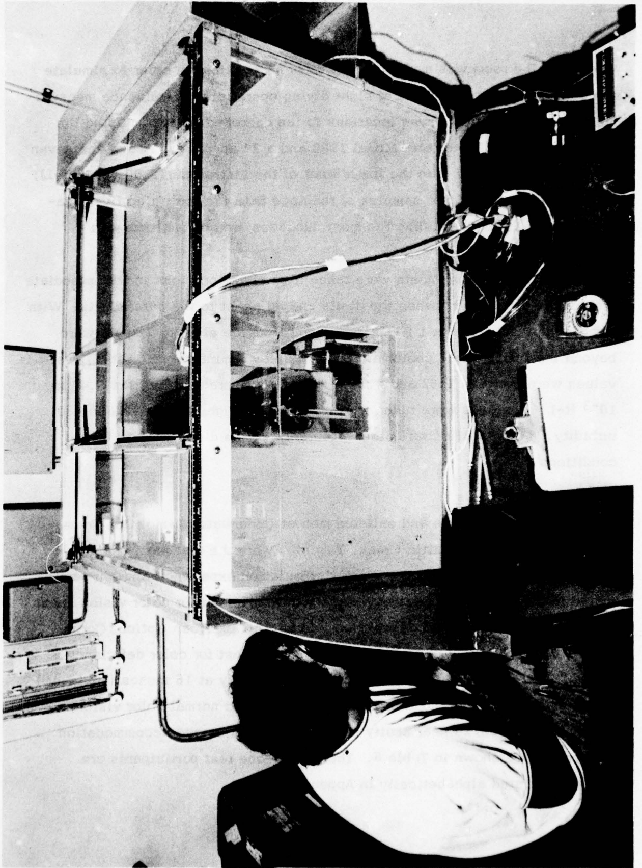
Figure 6. Test Tank and Drywell Apparatus
