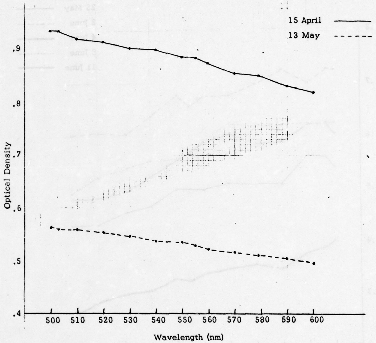
Figure 8. Optical Density vs Wavelength for Two Samples of Harbor-10 Turbidity
