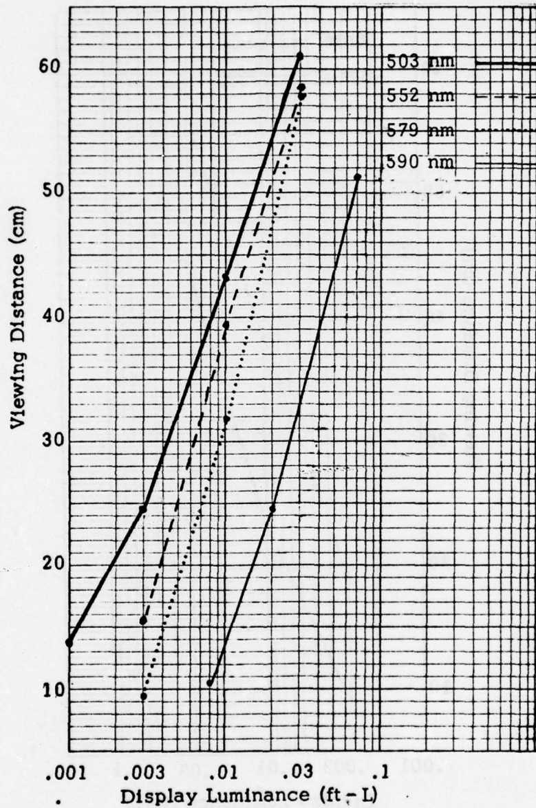
Figure 20. Maximum Legible Viewing Distance in Ocean Turbidity as a Function of Display Wavelength
