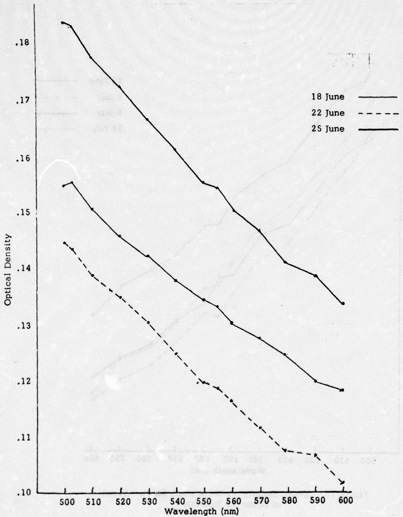
Figure 11. Optical Density vs Wavelength for Three Samples of Ocean-30 Turbidity
