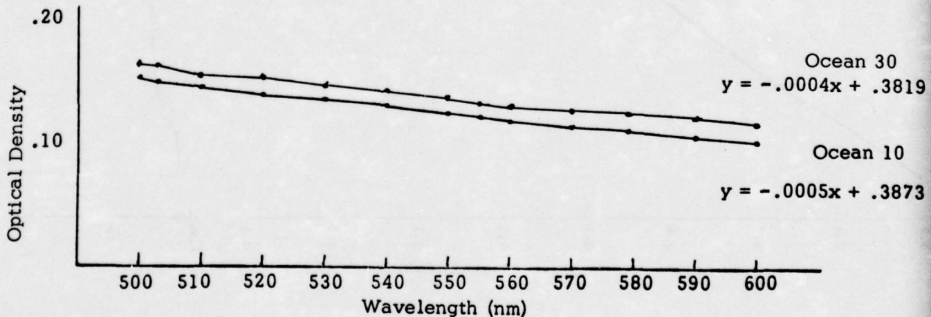
Figure 13. Optical Density of Artificially Turbid 'Ocean' Water
