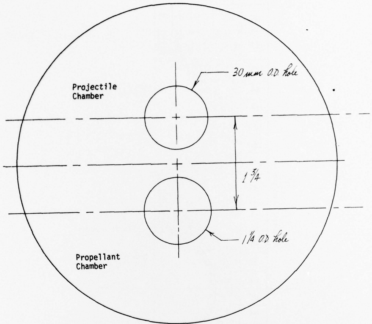
Figure 15. Representative Cross Section of the Gun Tube Chamber
