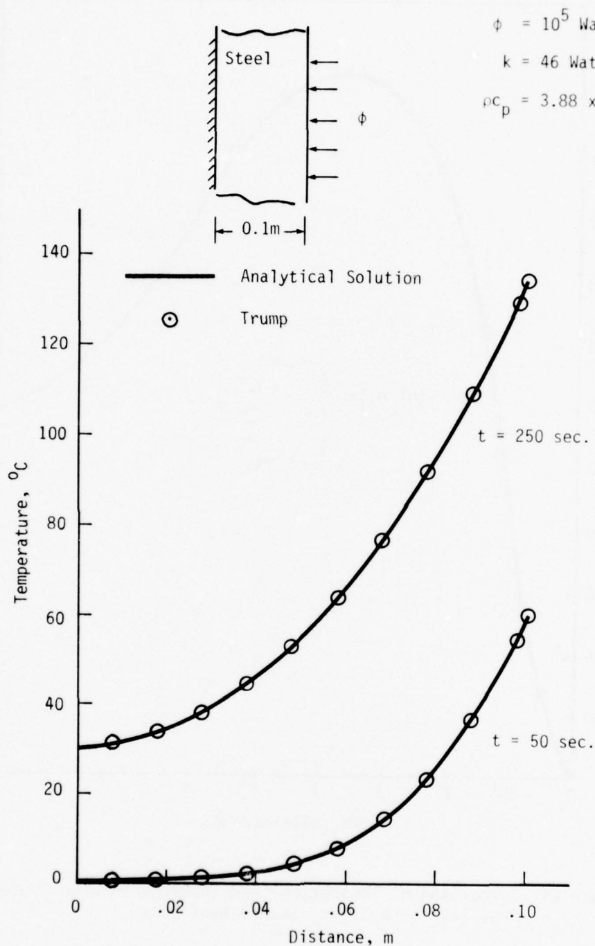
Figure 12. Comparison of Theoretical and TRUMP Calculated Temperature Profiles for a Rectangular Slab with a Constant Heat Flux on One Face and Insulated at the Other
