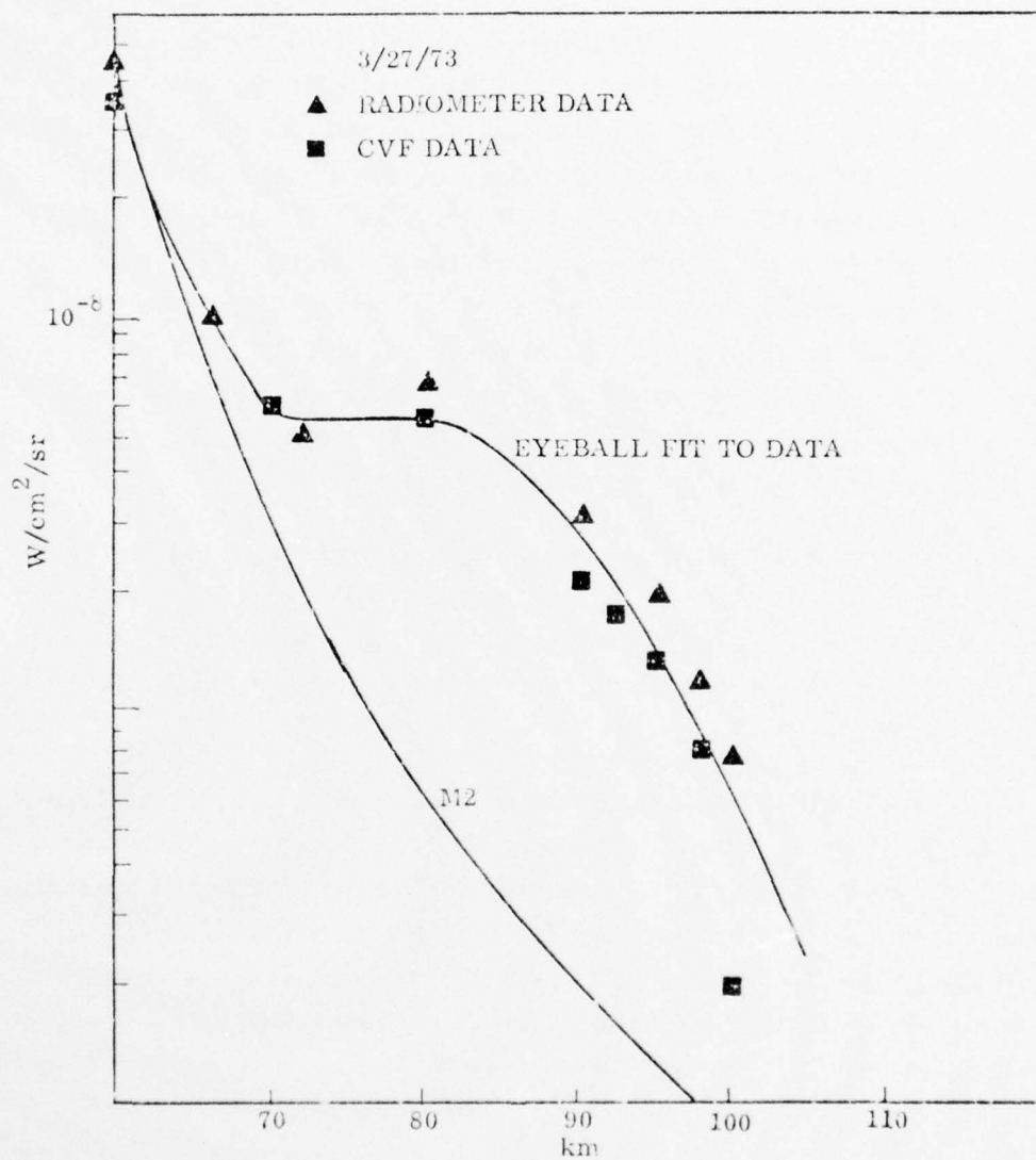
Figure 5. Auroral 4.3 \mu\text{m} zenith radiance data obtained on the downleg of a rocket experiment (Stair et al., Reference 2) conducted on 27 March 1973 are compared with an ambient night time radiance calculation (curve M2). The model atmosphere on which the ambient calculation is based is described by Kumer (Reference 15).
