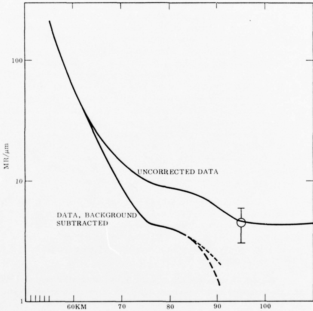
Figure 6. Preliminary version of 4.3 μm zenith radiance data obtained on 11 April 1974 under quiet conditions.
