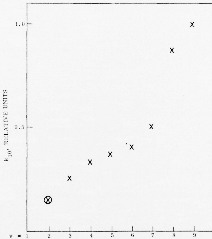
Figure 9a. The X's are data for k_{10}(v) from Reference 23. The \otimes is the extrapolated value of k_{10} for V = 2 .
