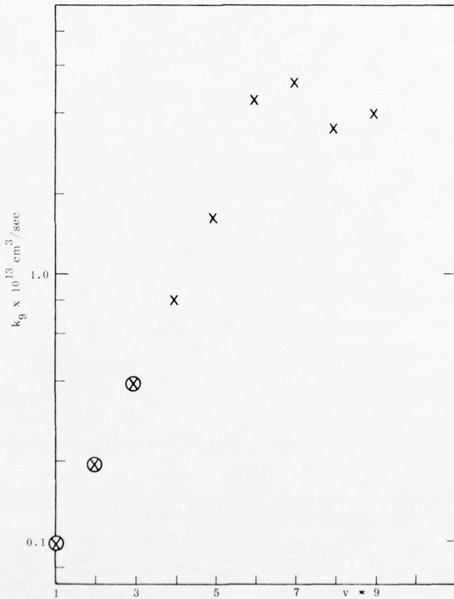
Figure 9b. The X's are data for k_g(\nu) from Reference 24. The \otimes 's are the extrapolated values we used for k_g(\nu) for \nu < 4 .
