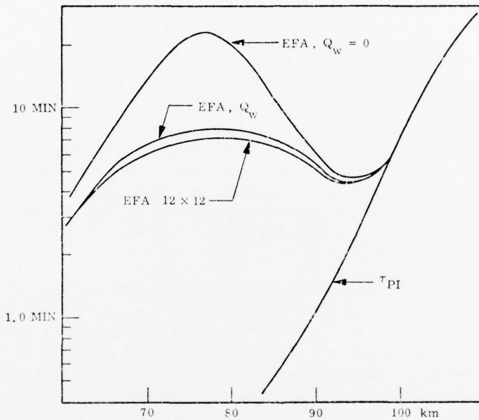
Figure 1. A comparison of the EFA estimates for the N_2^{\ddagger} relaxation time \tau . The curves labeled EFA, Q_w and EFA 12 x 12 include the effects of the weak CO_2 v_3 bands, the curve labeled EFA, Q_w = 0 does not. The curve labeled \tau_{PI} is the result one achieves by neglecting the vv transfer from CO_2 back to N_2 .
