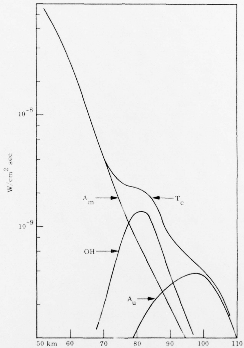
Figure 17. Curve T_c is our preliminary prediction for the 12 March 1975 upleg 4.3 \mu m zenith radiance profile.
