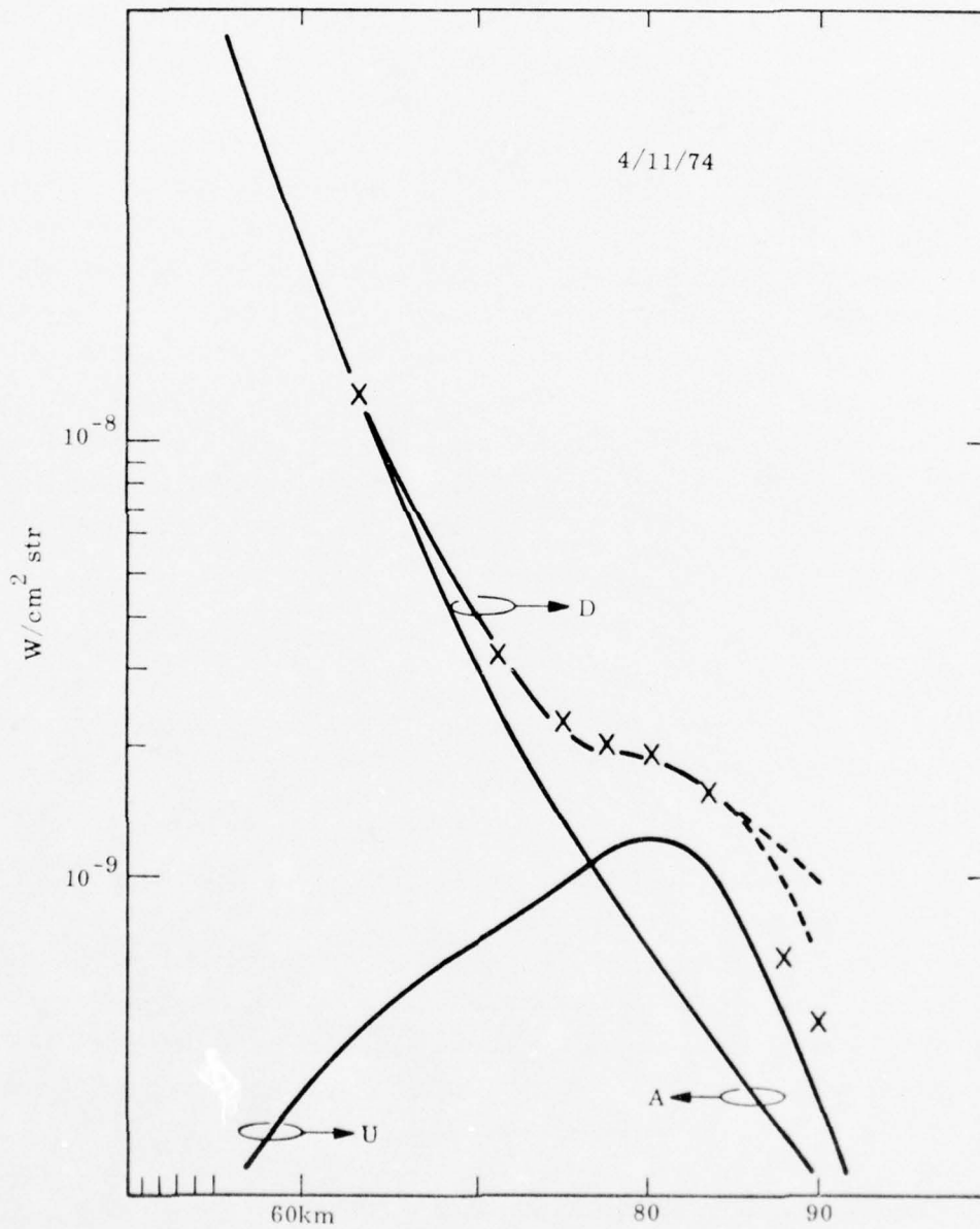
Figure 11. D, The 11 April 1974 data reduced by a factor 0.63 A, Ambient calculation U, The OH component, it requires OH + transfers .078 ergs/cm 2 sec to M 2 + X, The fit A + U to the data D
