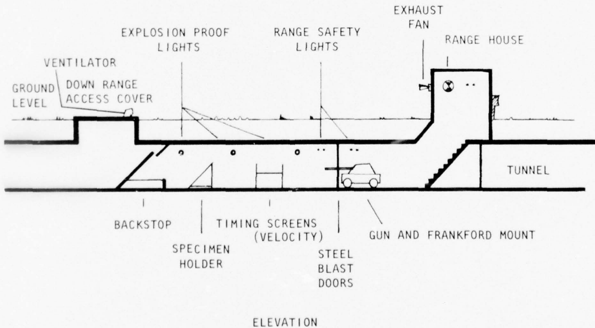
Figure V-1. Boeing Vertol Ballistic Test Facility.
