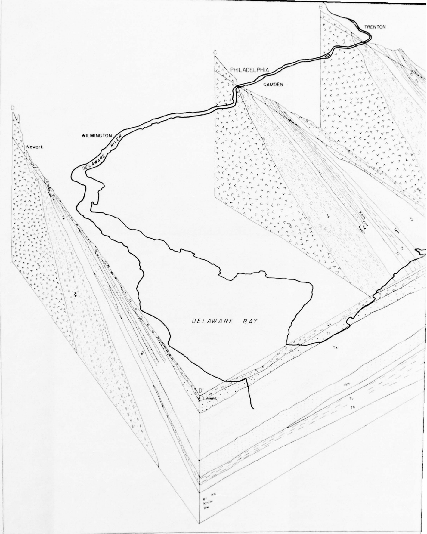
FENCE DIAGRAM OF COASTAL PLAIN IN DELAWARE RIVER B
