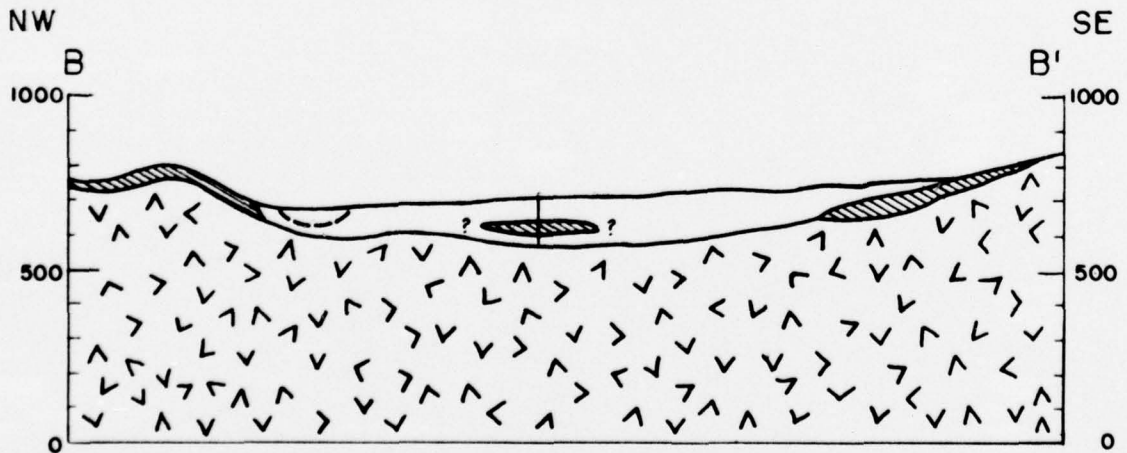
Geologic section B-B' across Delaware River, Narrowsburg, Sullivan County, N.Y.
