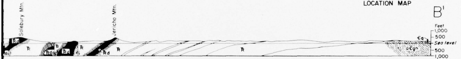
From Greenman, D.W., 1955, Ground Water Resources of Bucks County, Pa. Geol. Sur. Bull. W-11, pl. I.
