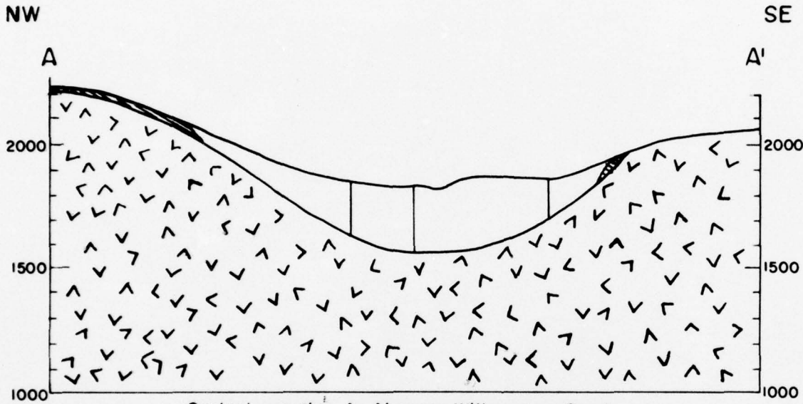
Geologic section A-A' across Willowemoc Creek, Willowemoc, Sullivan County, N.Y.
