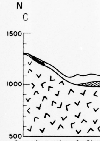
Geologic section C-C' across Delaware River, Downsville.
