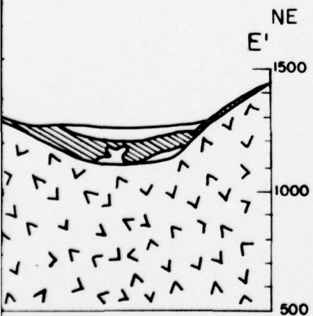
Geologic section E-E' across Neversink River, Godeffroy, Sullivan County, N.Y.
