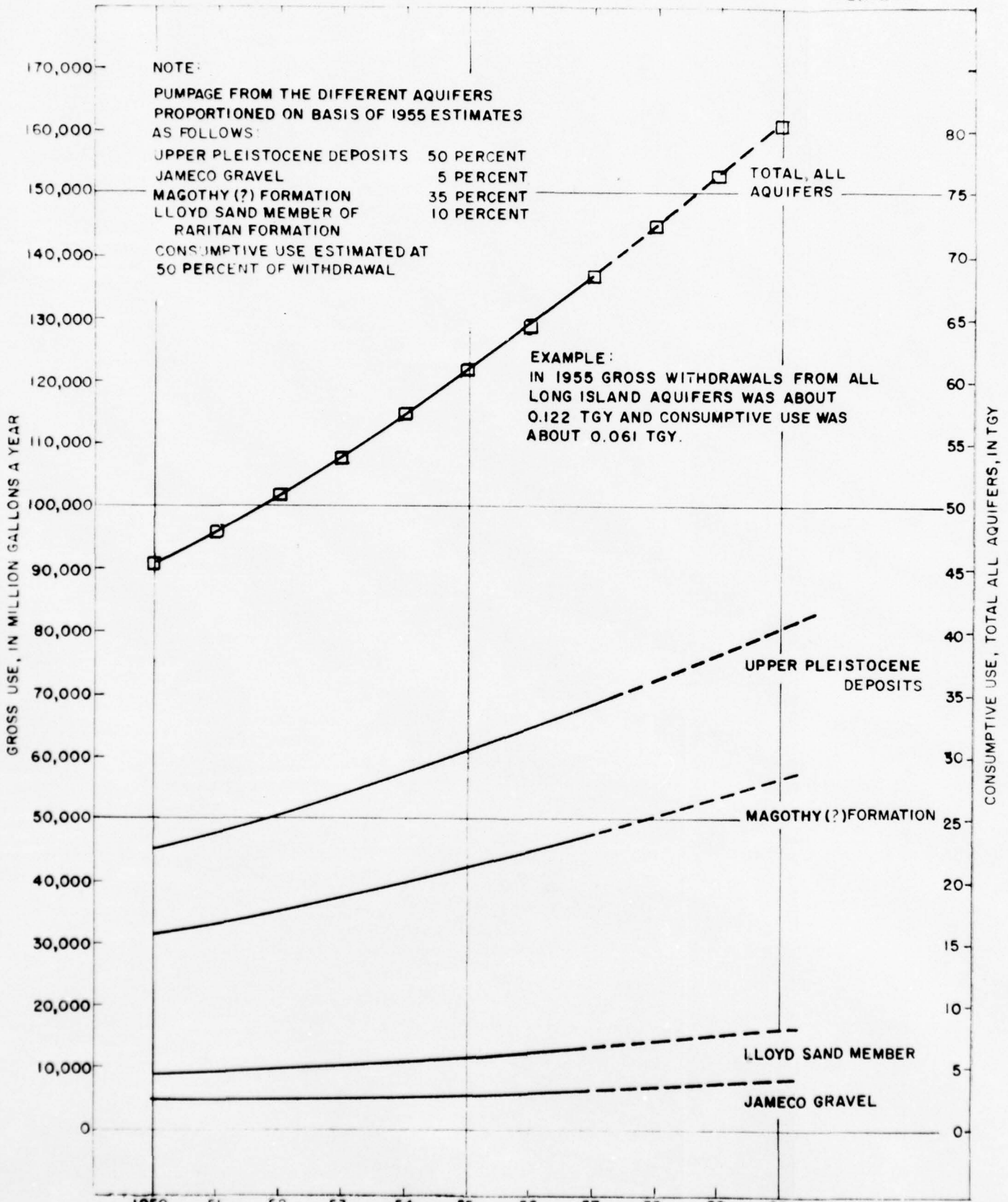
GRAPH SHOWING PUMPAGE AND CONSUMPTIVE USE FROM AQUIFERS OF LONG ISLAND, N.Y., 1950-1957, PROJECTED TO 1960
