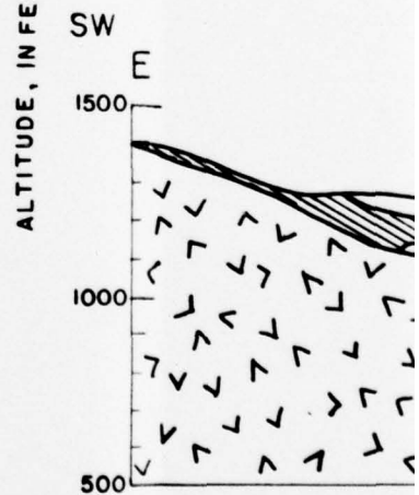
Geologic section E-E' across Neversink, Sullivan County, N.Y.
