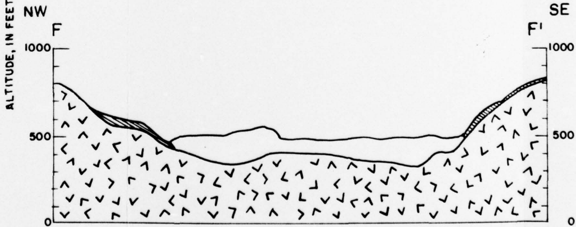
Geologic section F-F' across Neversink River, Godeffroy, Orange County, N.Y.
