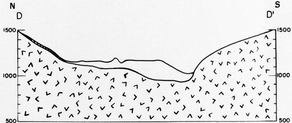
Geologic section D-D' across West Branch Delaware River, Cannonsville, Delaware County, N.Y.
