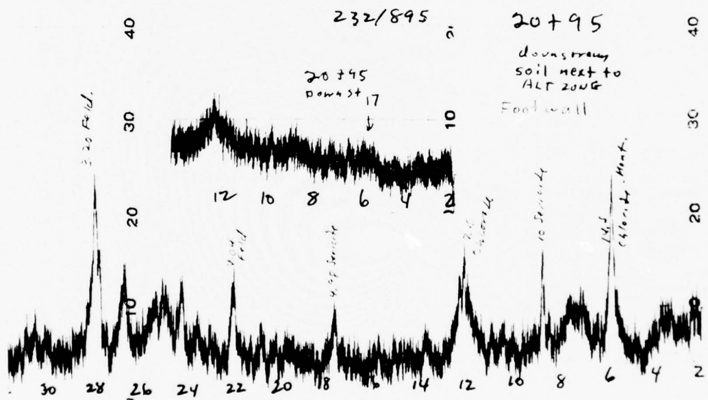
Plate 8. X-ray diffractograms of powder press samples of soil adjacent to altered felsite zone at station 20+95 (right of centerline) in west bank of diversion channel at Richard B. Russell project. (SAD Lab. No. 232/894 and 232/895)
