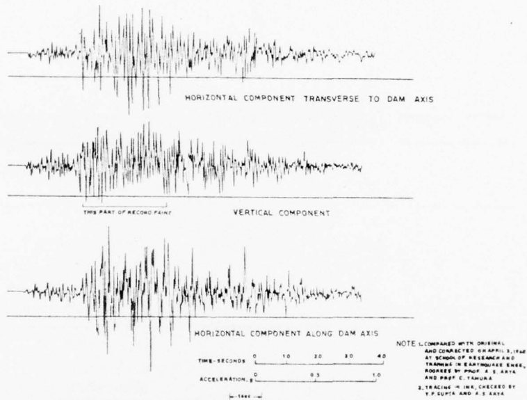
FIG. 1. Accelerogram Recorded at Block 1-A of Koyna Dam on December 11, 1967 at 04:21 I.S.T.
