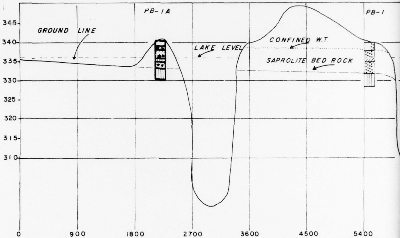
SECTION ALONG A-A' GRID EAST OF A SCALE IN FEET
