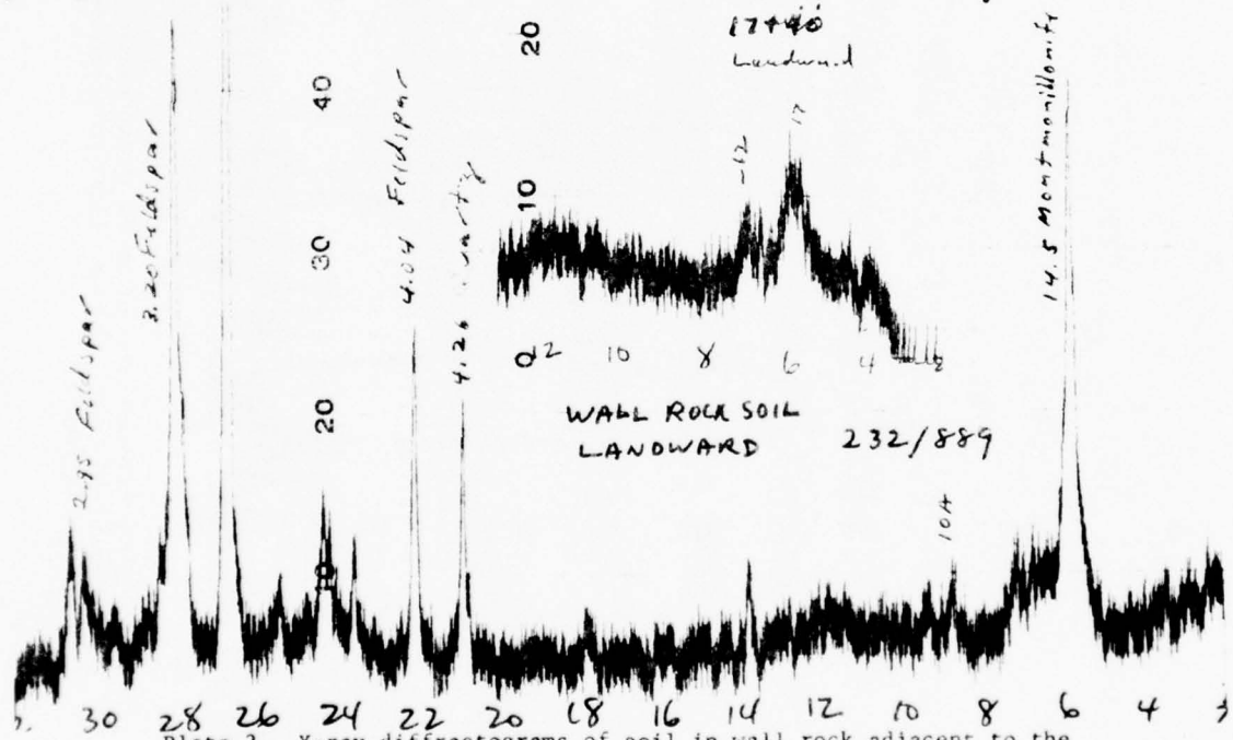
Plate 3. X-ray diffractograms of soil in wall rock adjacent to the altered felsite zone at station 17+40 (right of centerline) in diversion channel, Richard B. Russell Project. (SAD Lab. Nos. 232/888 and 232/889).
