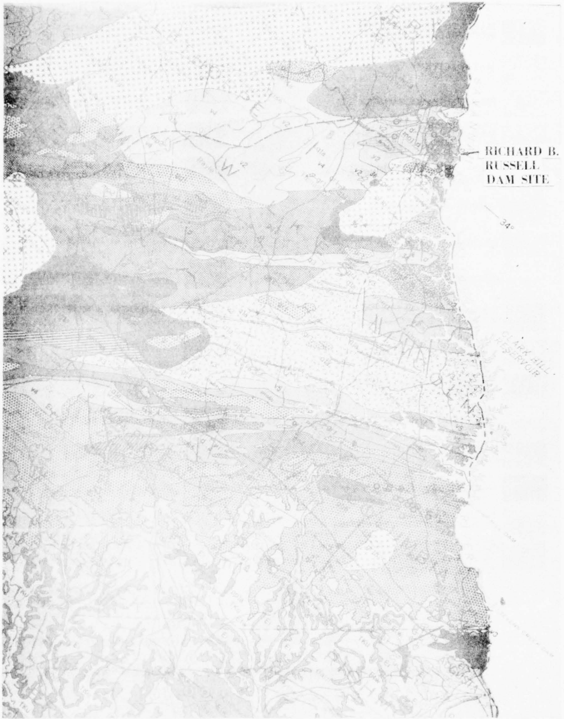
Figure 5 Portion of the Geologic Map of Georgia
