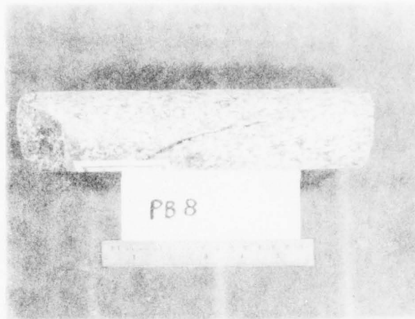
Figure 3. Hornblende gneiss from 54.5 to 55.2 feet depth of boring PB-8, Patterson Branch Seismic Zone. Dark lined minerals consist of hornblende biotite and chlorite in a groundmass of feldspar and quartz. The genetic classification of this rock unit is hornblende granodiorite gneiss. (SADL 232/941).
