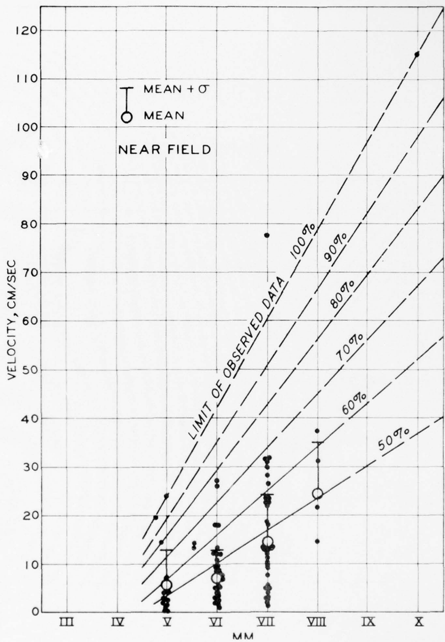
Velocity Versus MM Intensity in the Near Field. Also Shown is the Mean, Mean plus One Standard Deviation, and 10 percent Increments Between the Projected Mean and the Limit of Observed Data (Krnitzsky and Chang).
