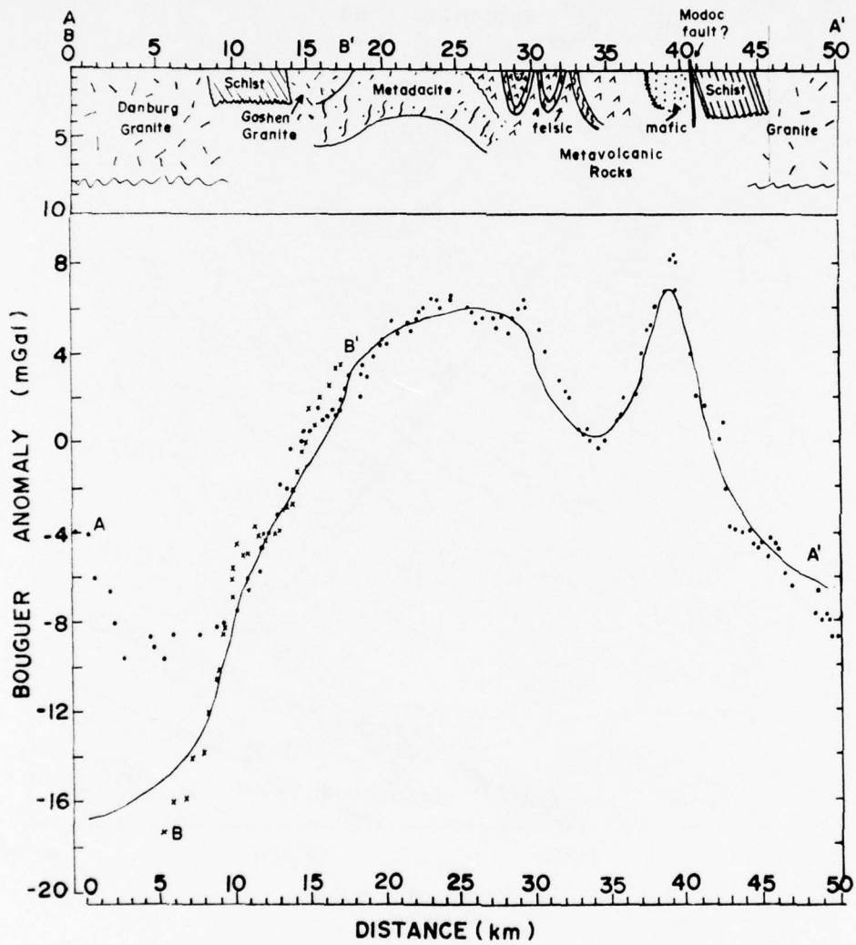
Figure 10. Profile AA' showing model used to explain Bouguer anomalies and hypothetical geological structure based on gravity model.
