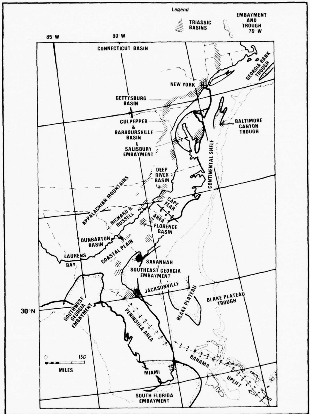
Map of the Atlantic Coastal Plain and Continental Shelf
