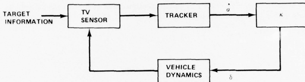
STABILIZED SEEKER
