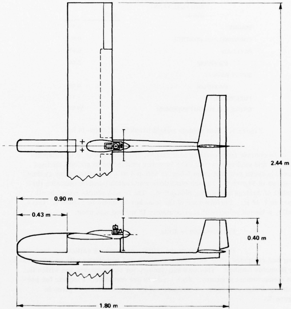
Figure 3. Test vehicle general arrangement for Phase I.
