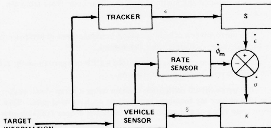
STRAP-DOWN SEEKER
