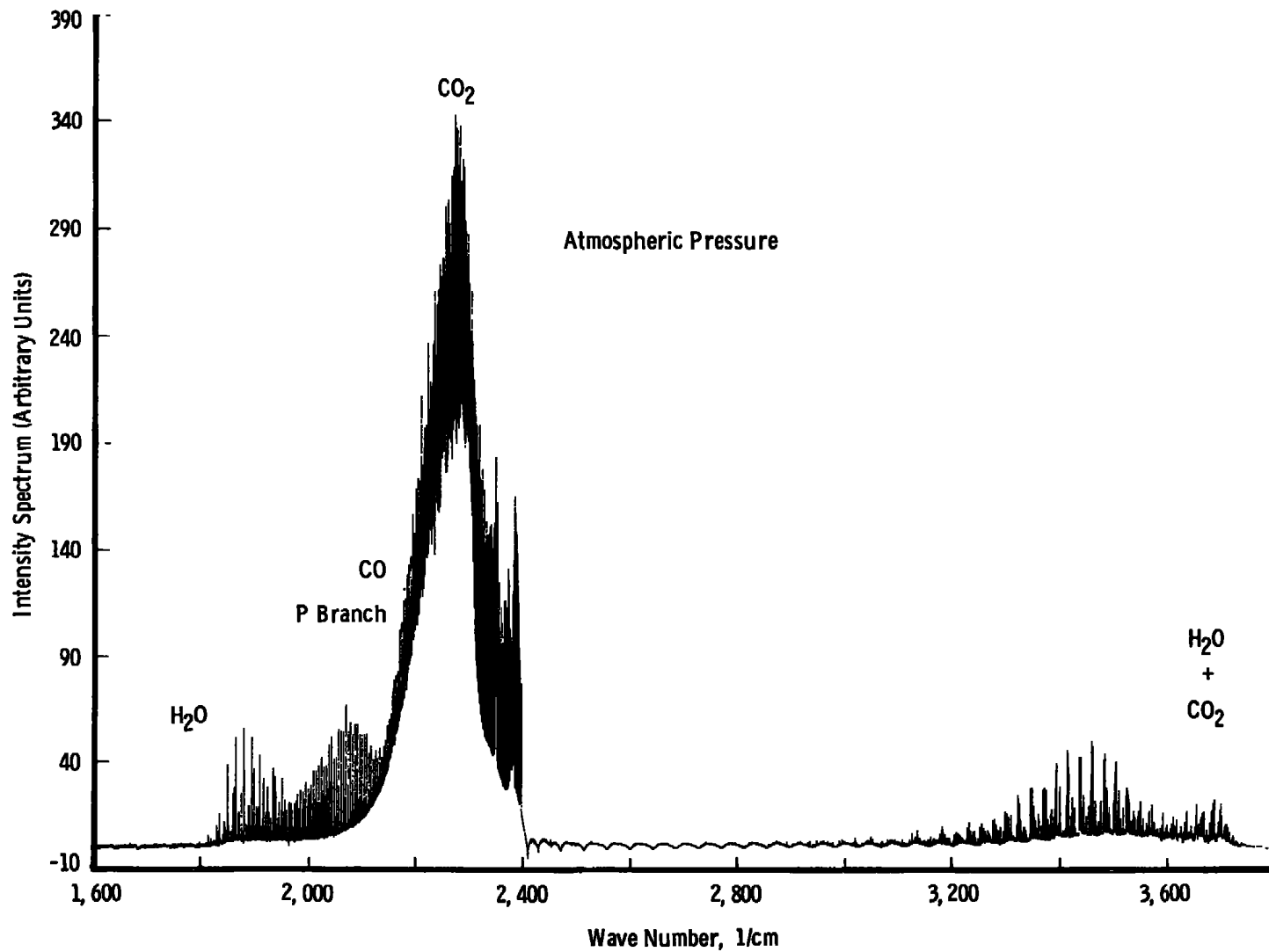
Figure 4. Emission spectrum of benzomatic torch (1,800 to 3,700 \text{cm}^{-1} , 0.2 \text{cm}^{-1} resolution).
