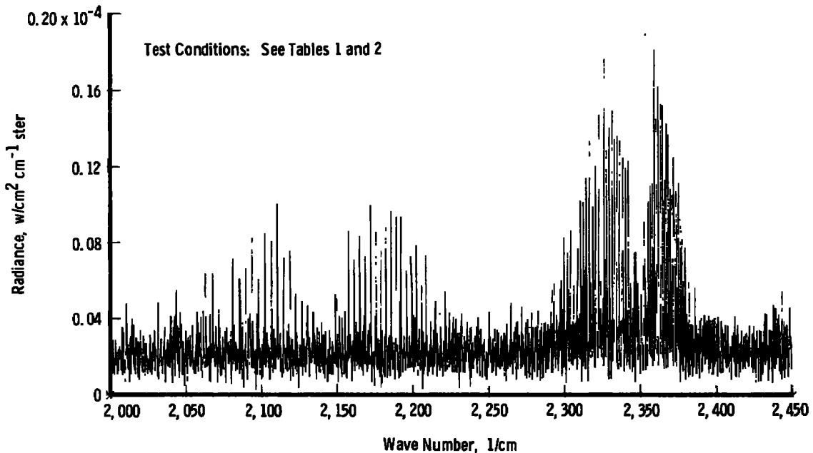
Figure 8. Emission spectrum of rocket plume in R-2H Test Cell (2,000 to 2,450 cm -1 , 0.3 cm -1 resolution).
