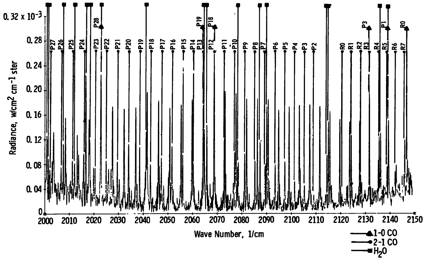
Figure 7. Emission spectrum of rocket plume in T-3 Test Cell (2,000 to 2,150 cm^{-1} , 0.3 cm^{-1} resolution).
