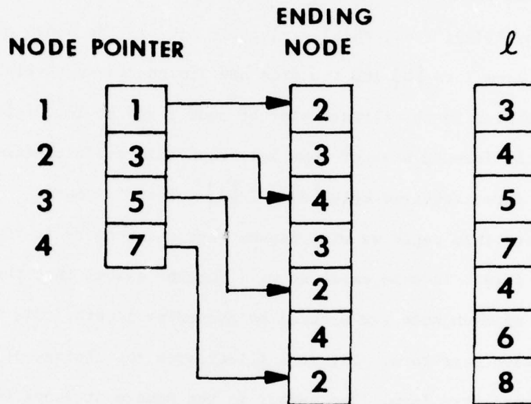
FIG. 1 - SORTED FORWARD STAR FORM
