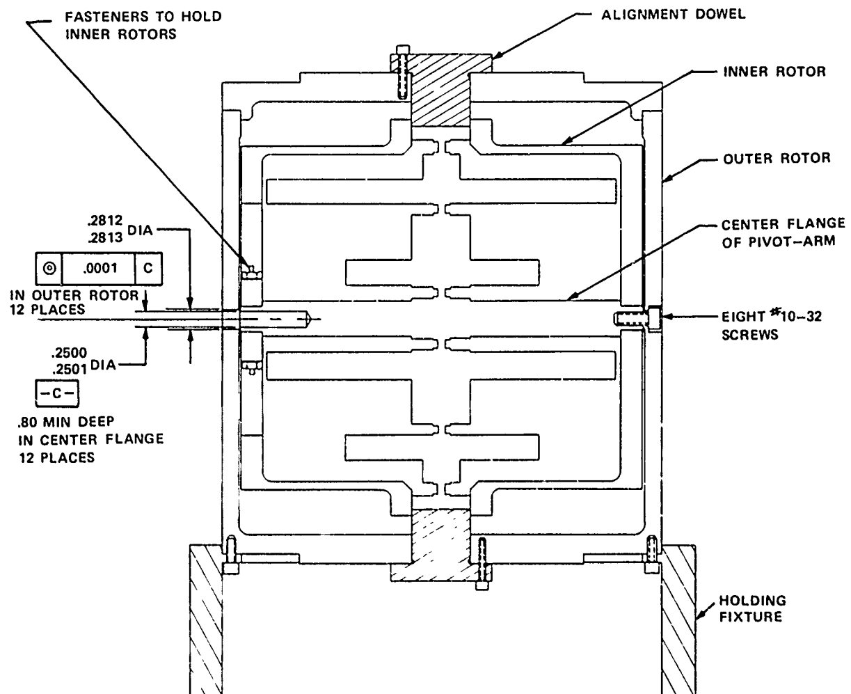
Figure 2-31. Rotor match-boring.
