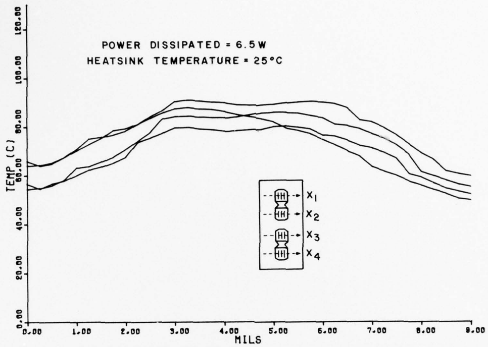
Figure 11. Uneven temperature distribution - TA8791 transistor.
