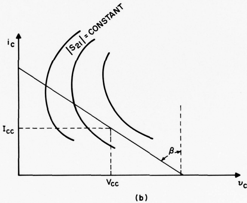
Figure 17. Load line for linear operation.
