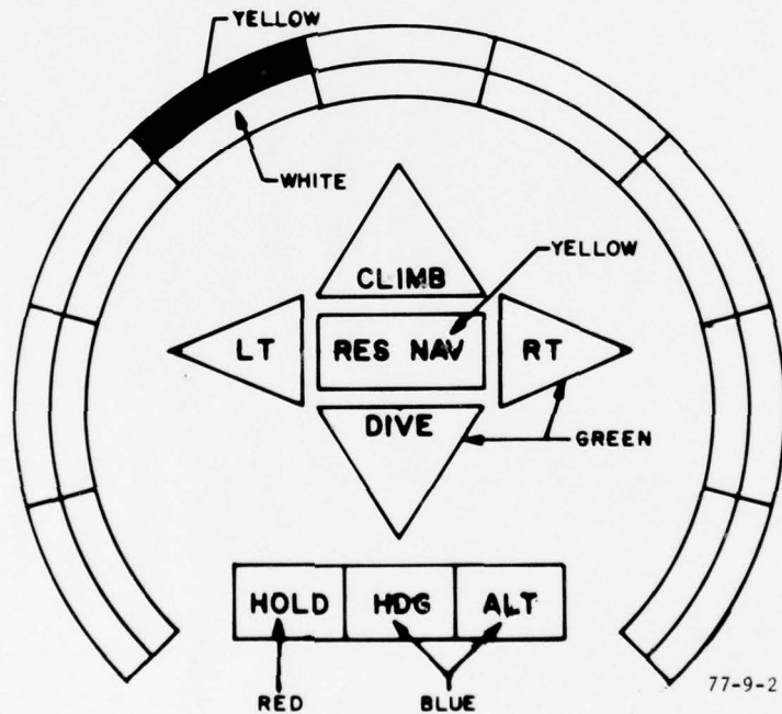
FIGURE 2. THE NAFEC-PROPOSED IPC DISPLAY
