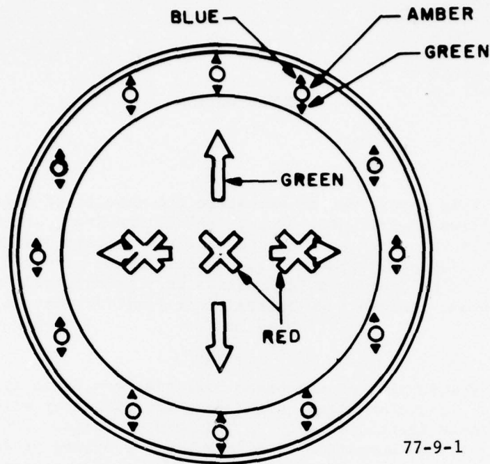
FIGURE 1. THE BADCOM IPC DISPLAY
