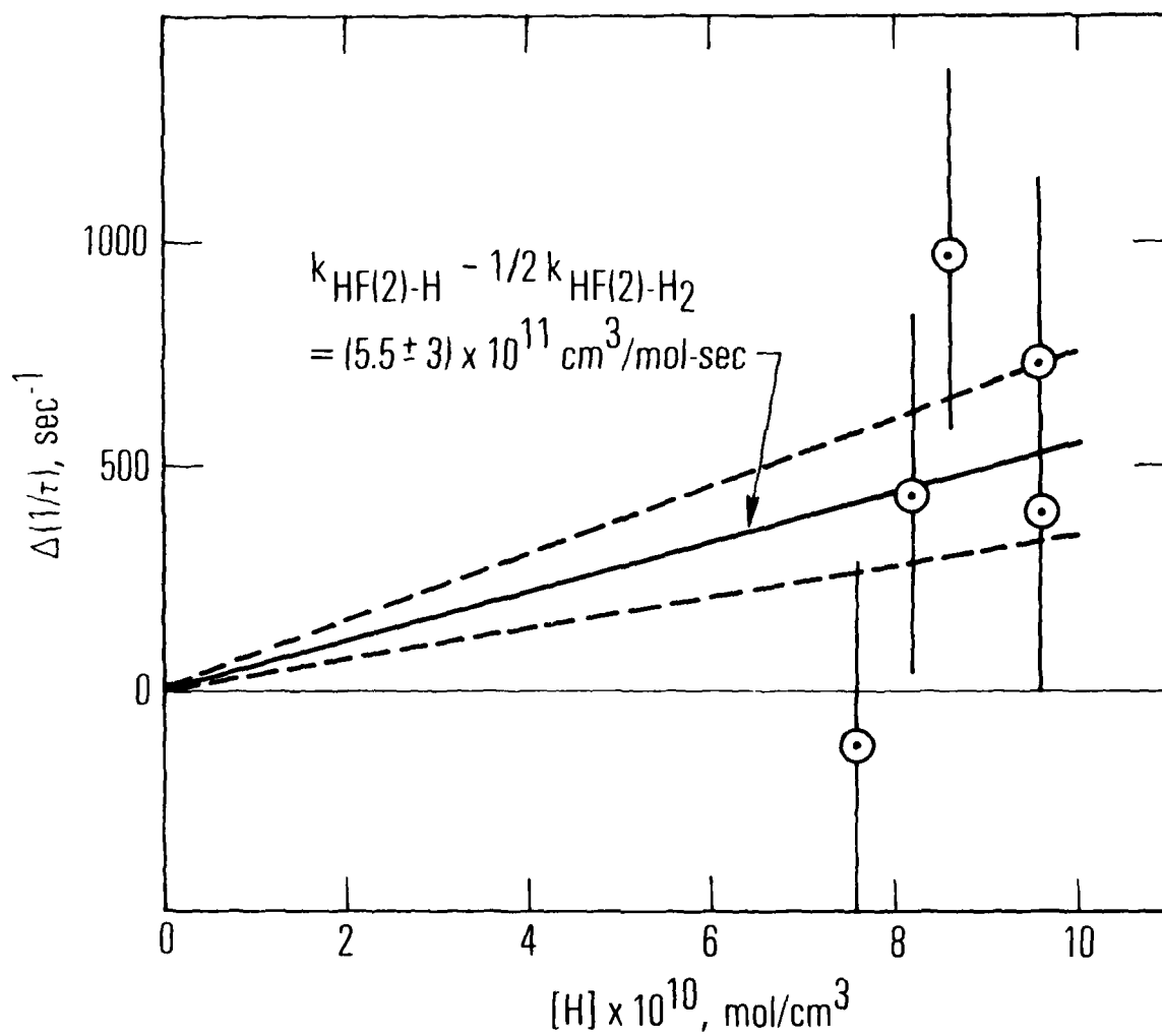
Figure 3. Removal Rates of HF(v = 2) by H Atoms
