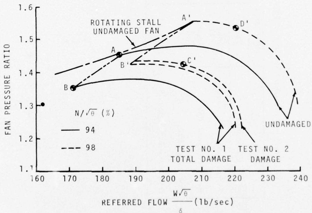
Figure 71. Scaling Procedure for Damaged Fan Efficiency and Pressure Ratio Maps.
