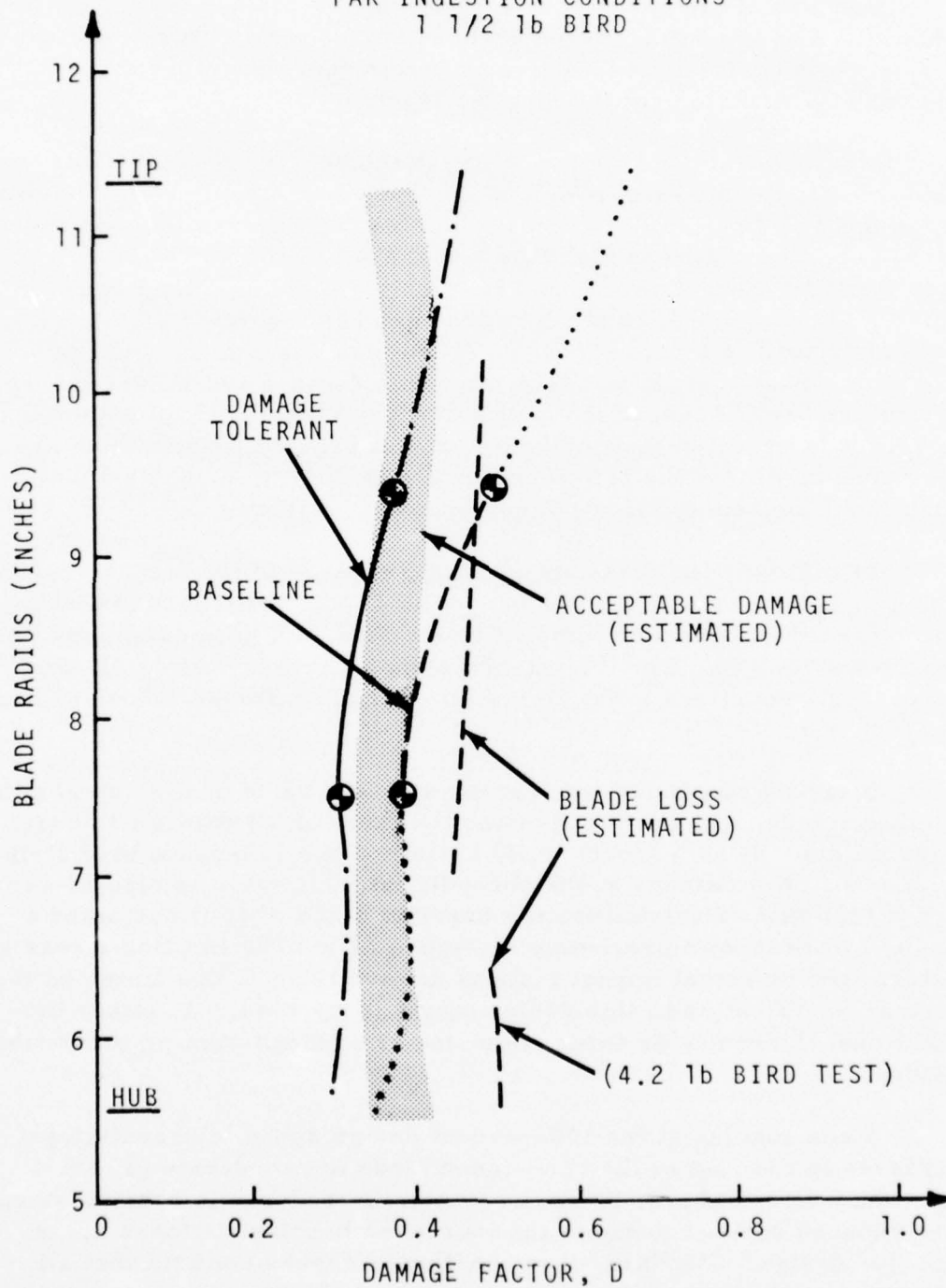
Figure 87. Redesign of Damage Factor Limits - 1600 lbf Blade.
