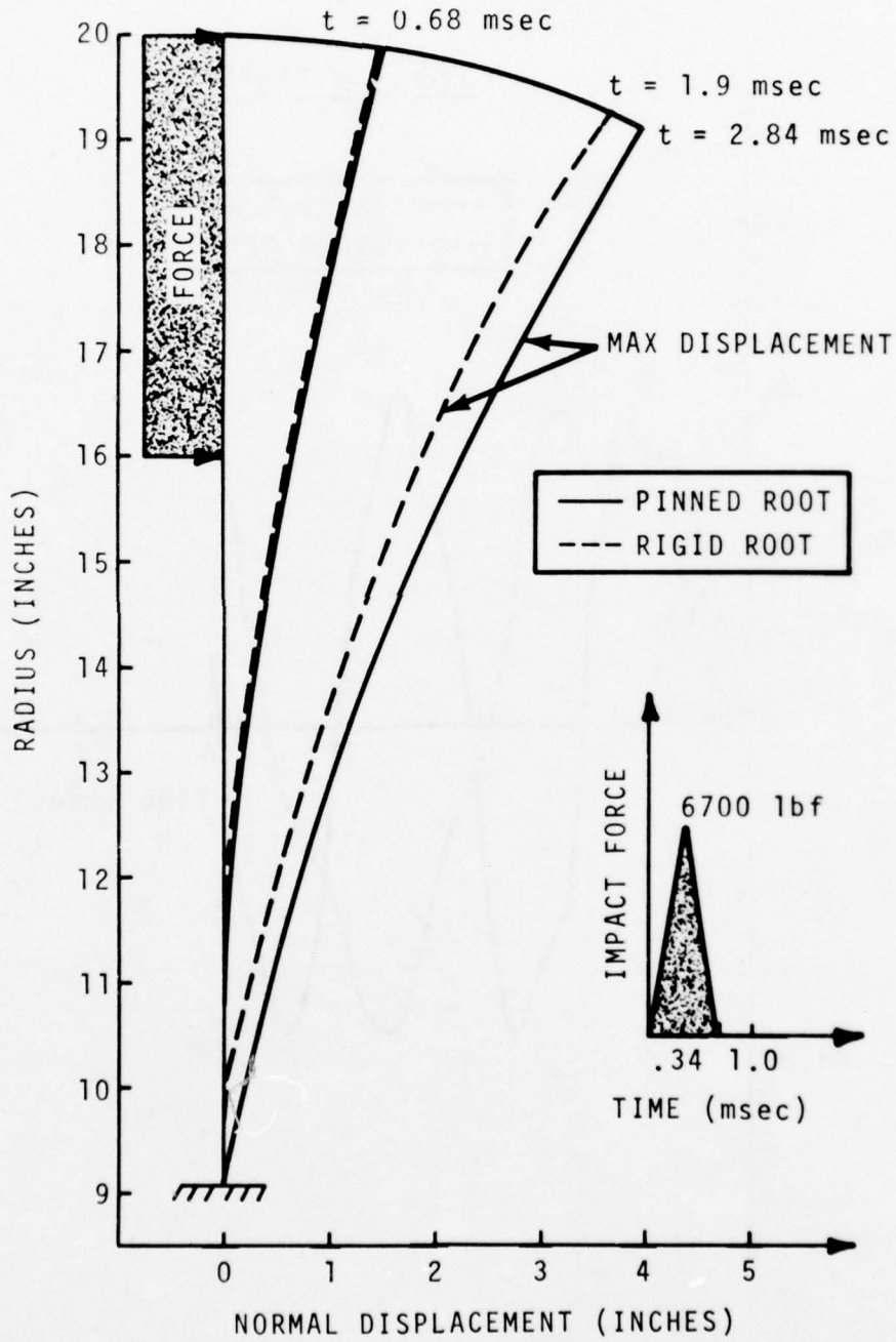
Figure 61. Effect of Pinned Root on Transient Deformation - 6800 lbf Blade.
