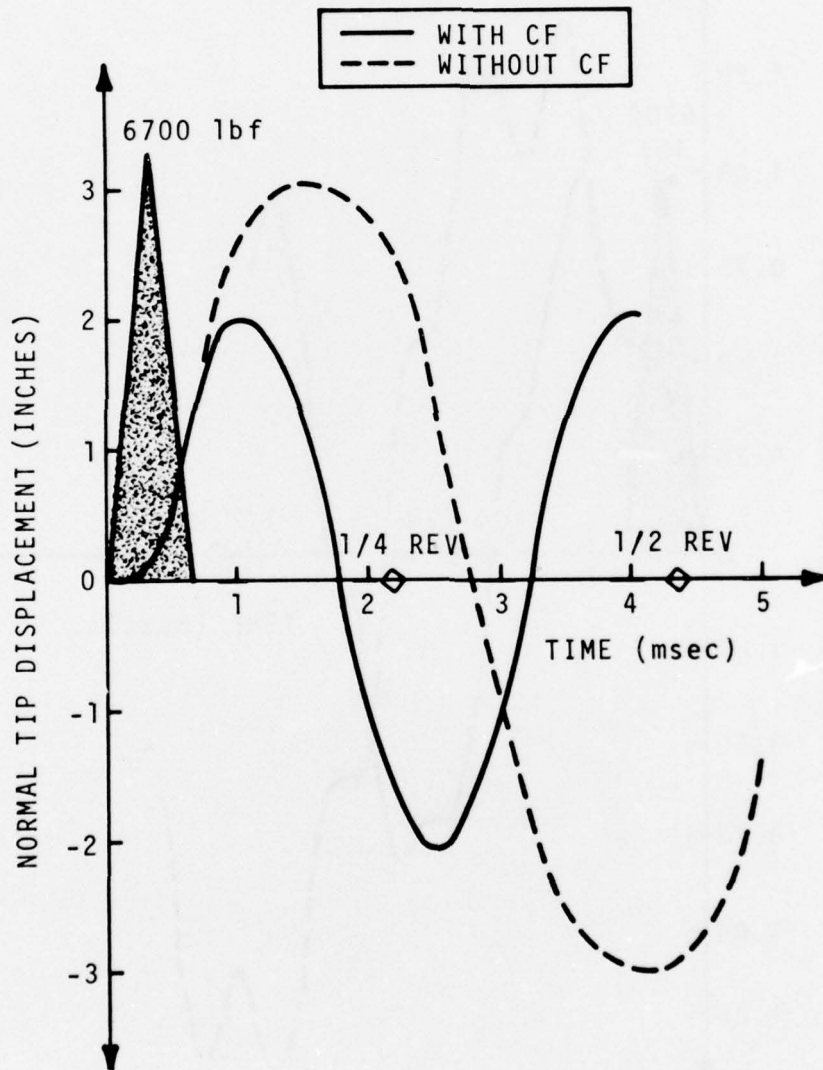
Figure 47. Centrifugal Force Effects on Tip Displacement - 6800 lbf Baseline Blade.
