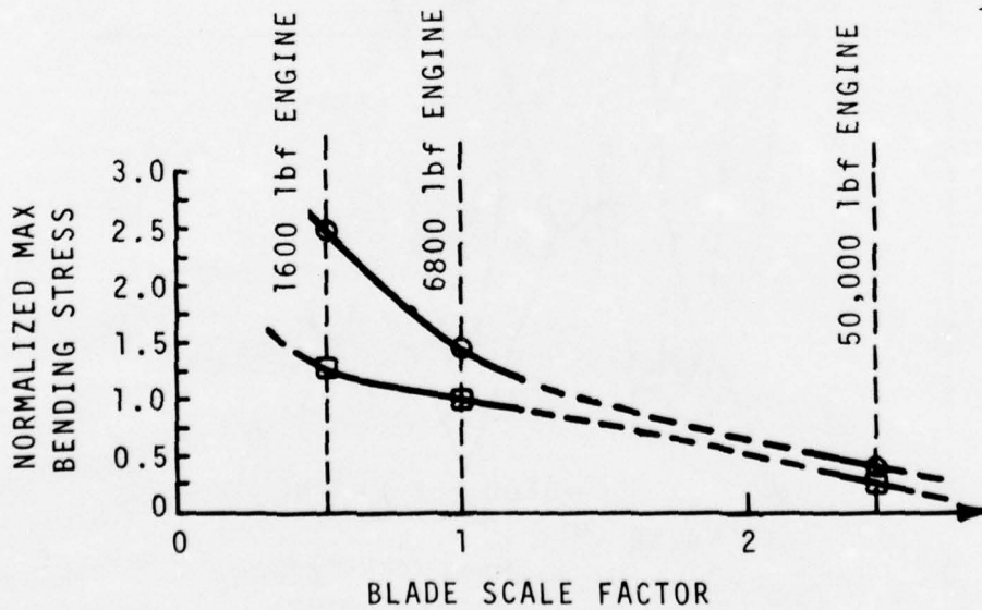
Figure 54. Tip Displacements and Maximum Stresses Versus Blade Scale Factor.
