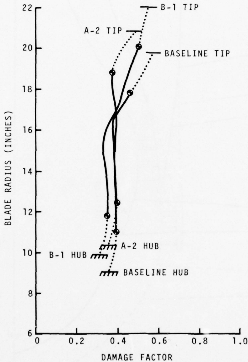
Figure 68. Damage Factor Comparison of Alternate Fan Designs - 6800 lbf Engine.
