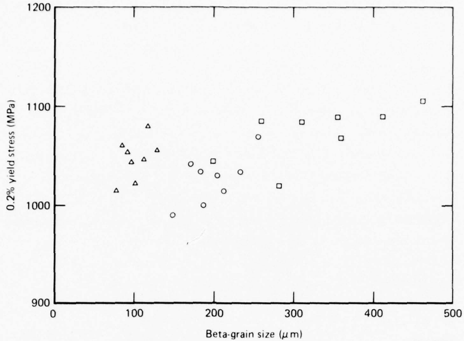
Figure 23. Dependence of yield stress on beta-grain size for (□) Ti-6Al-4V reference alloy, (○) Ti-6Al-4V-0.020Y, and (Δ) Ti-6Al-4V-0.10Er.
