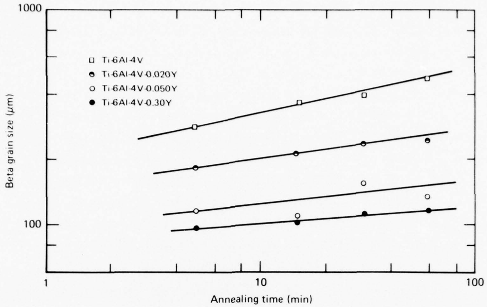
Figure 11. Beta grain size as function of annealing time at T_{\beta} + 56^{\circ}\text{C} for (□) Ti-6Al-4V reference alloy, (●) Ti-6Al-4V-0.020Y, (○) Ti-6Al-4V-0.050Y, and (●) Ti-6Al-4V-0.30Y.
