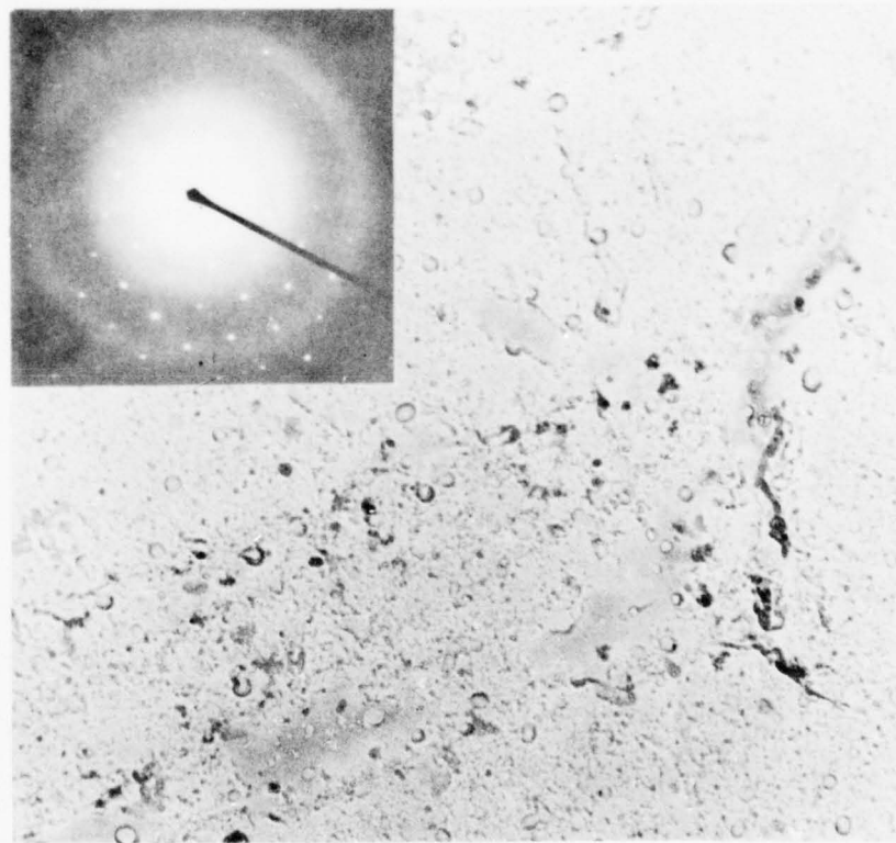
Figure 8. Electron micrograph of carbon-extraction replica of dispersoids in Ti-6Al-4V-0.30Y; inset shows electron diffraction pattern of single dispersoid.
