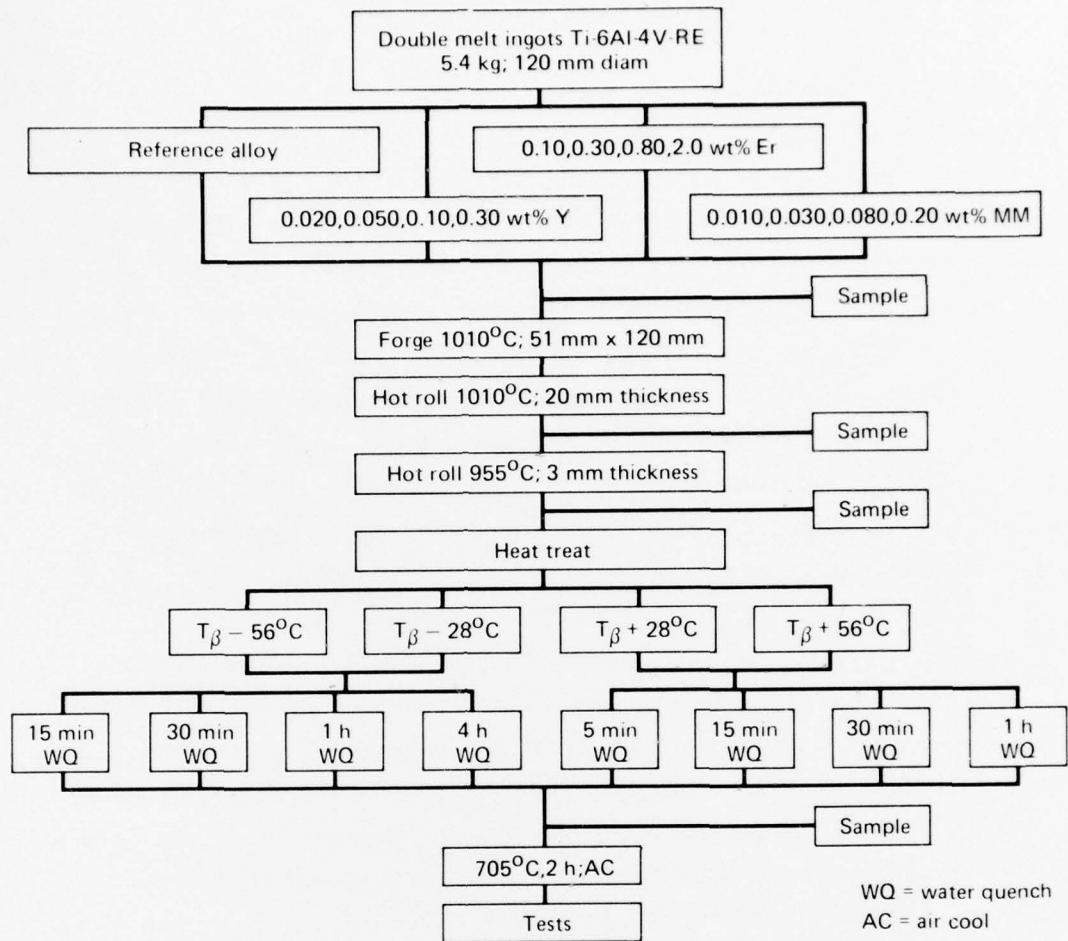
Figure 1. Outline of alloy preparations and heat treatments for study of microstructures and room-temperature tensile properties of Ti-6Al-4V alloys with erbium, yttrium, and mischmetal additions.
