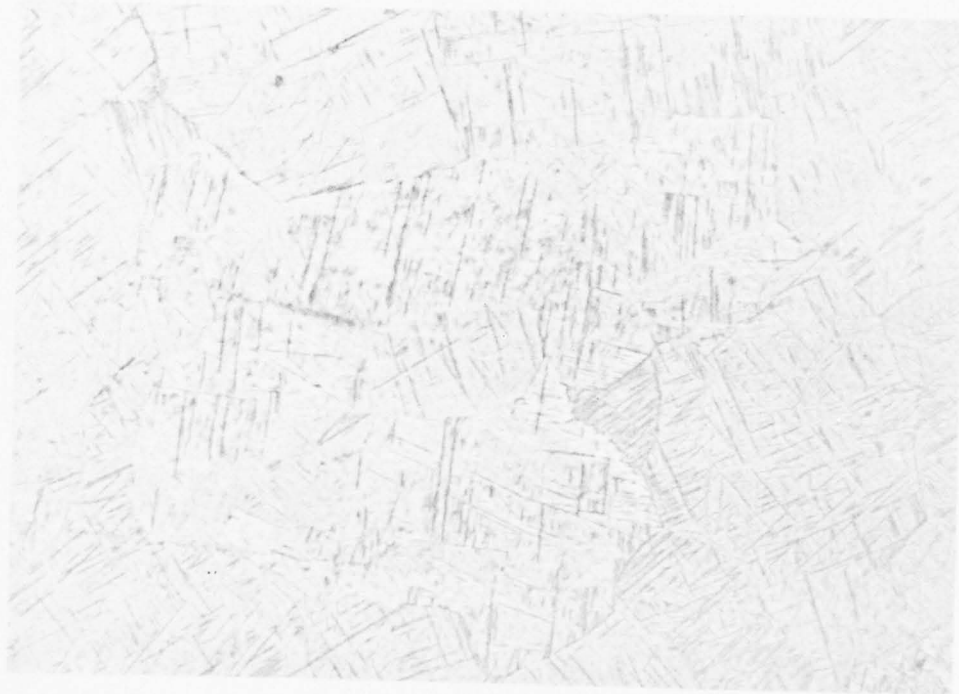
Figure 9. Microstructures of beta-annealed (a) Ti-6Al-4V reference alloy and (b) Ti-6Al-4V-0.30Y; alloys annealed at T_{\beta} + 56^{\circ}\text{C} for 5 min and water-quenched.
