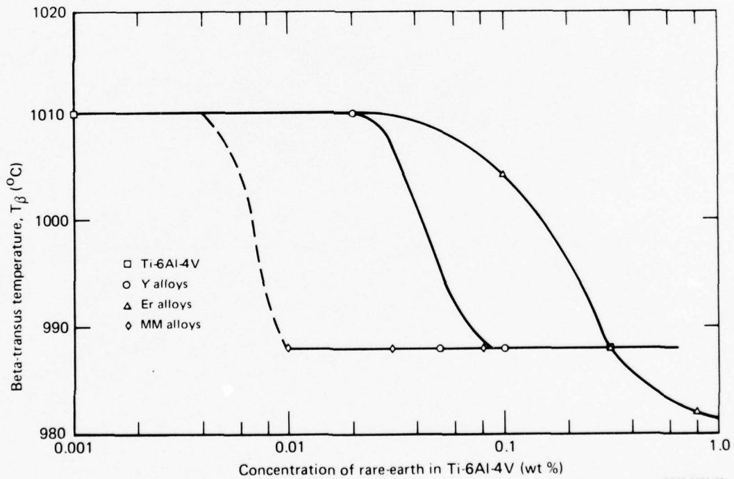
Figure 4. Ti-6Al-4V beta-transus temperature as function of concentrations of added Y (○), Er (△), and MM (◇).
