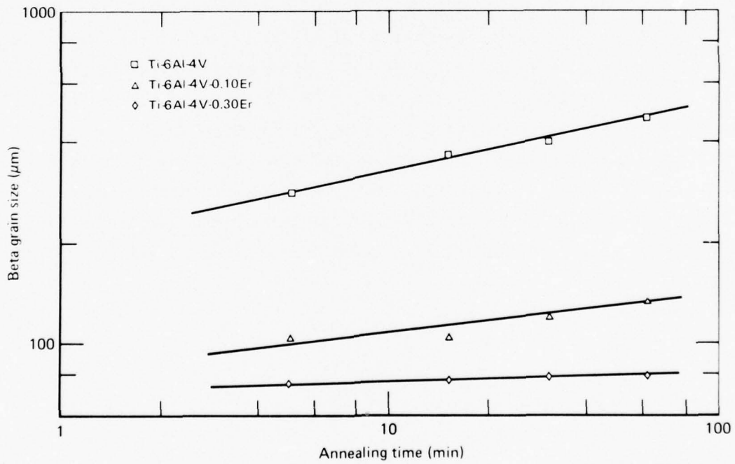
Figure 12. Beta grain size as function of annealing time at T_{\beta} + 56^{\circ}\text{C} for (□) Ti-6Al-4V reference alloy, (△) Ti-6Al-4V-0.10Er, and (◇) Ti-6Al-4V-0.30Er.
