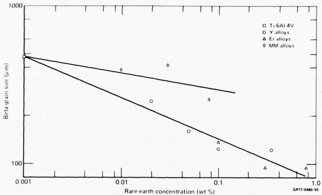
Figure 13. Beta-grain size as function of rare-earth concentration in Ti-6Al-4V-RE alloys annealed for 1 h at T_{\beta} + 56^{\circ}\text{C} ; (□) Ti-6Al-4V reference alloy, (○) Y additive, (△) Er additive, and (◇) MM additive.
