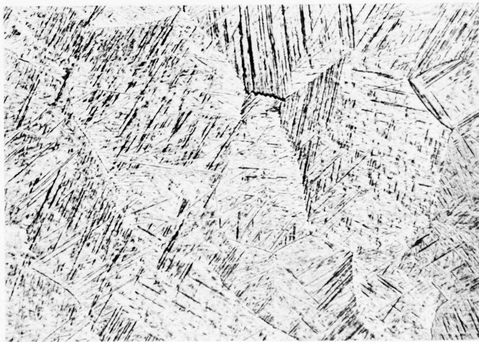
Figure 10. Microstructures of beta-annealed (a) Ti-6Al-4V-0.80Er and (b) Ti-6Al-4V-0.080MM; alloys annealed at T_{\beta} + 56^{\circ}\text{C} for 5 min and water-quenched.
