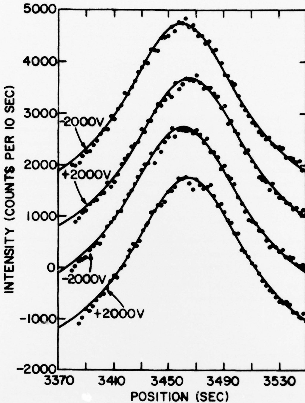
Figure 4. Line profile of (220) reflection of berlinite sample XP2 under the influence of an externally applied electric field of \pm 2000\text{V} . (The curves are displaced vertically in multiples of 100 counts/second)
