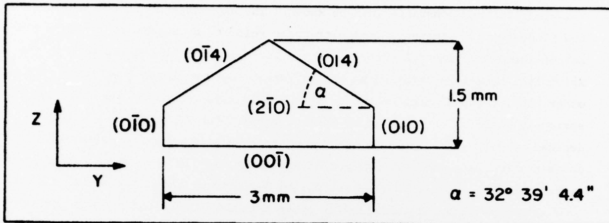
Figure 3. Dimensions, orientation and shape of X-cut platelet of berlinite sample XPl used for x-ray determination of piezoelectric constants. The plate thickness is 1.09 mm. The orientation of the right-handed cartesian coordinate system corresponds to the 1949 IRE convention (Proc. IRE 14 , 51, 1378-1395 (1949)). The pentagon shaped faces (2\bar{1}0) and (\bar{2}10) (equivalent to (\bar{1}\bar{1}0) and (110) , respectively) were electroded.
