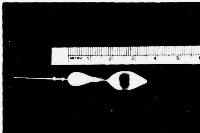
Figure 1. Typical Ba_2Ge_2TiO_8 Crystal Boule Pulled from Its Melt
