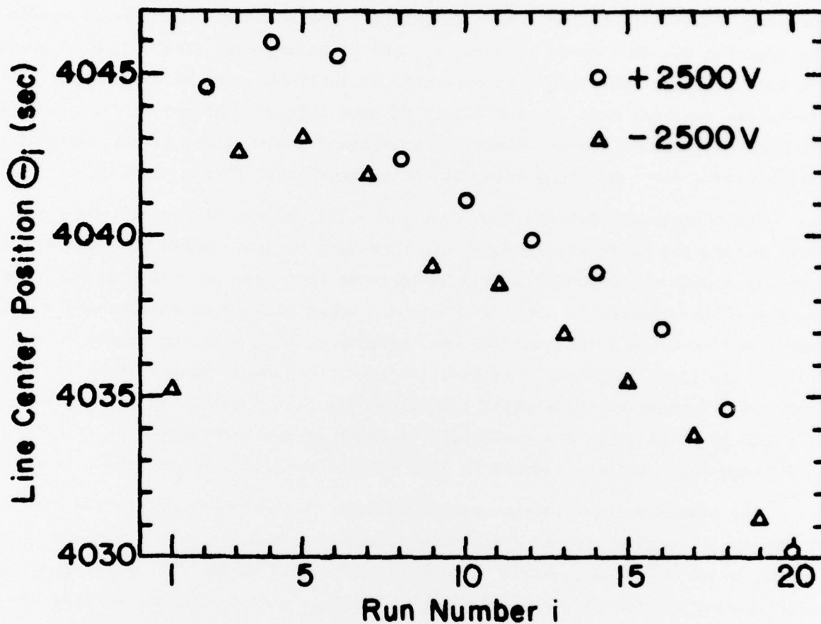
Figure 5. Line center position of (220) reflection of berlinite sample XP1 for successive runs under the influence of an externally applied electric field of \pm 2500V
