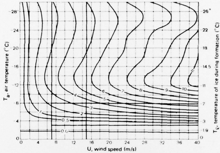
Figure B5. Amount of ice (g/h) which may form on a 1-cm 2 flat surface during ship icing under the following conditions: T_w = -1.7^\circ\text{C} , S = 34\text{ ‰} , L_z = 4.0 , L_i = 601 - 700 , C_q = 0.6 - 36.5 , C_w = 0.96 (Borisenkov et al. 1971).
