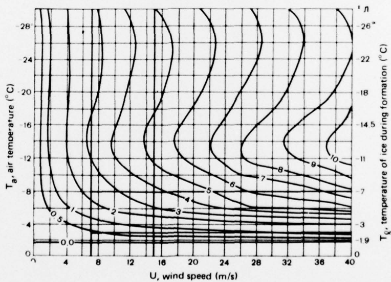
Figure B8. Amount of ice (g/h) which may form on a 1-cm 2 flat surface during ship icing under the following conditions: T_w = 2^\circ\text{C} , S = 34\text{‰} , L_z = 4.0 , L_i = 601 - 700 , C_q = 0.6 - 36.5 , C_w = 0.96 (Borisenkov et al. 1971).
