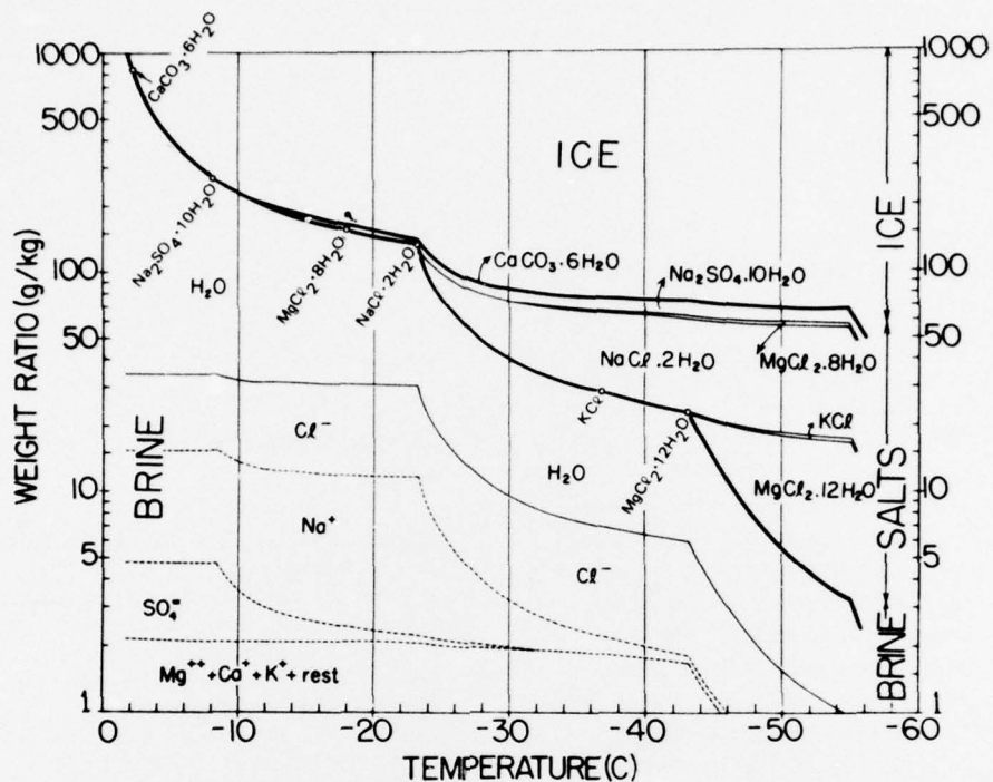
Figure 1. Phase relations for standard sea ice (Assur 1958).
