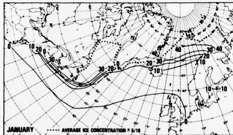
Figure A6. Moderate and severe potential superstructure icing for North Atlantic; November-January (DeAngelis 1974).
