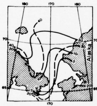
Figure A2. Probability (in percentage) of meteorological conditions conducive to the development of spray icing (combination of t_a < 0^\circ\text{C} and V > 8\text{ m/s} ) in September (—) and October (---), from Kolosova (1972).
