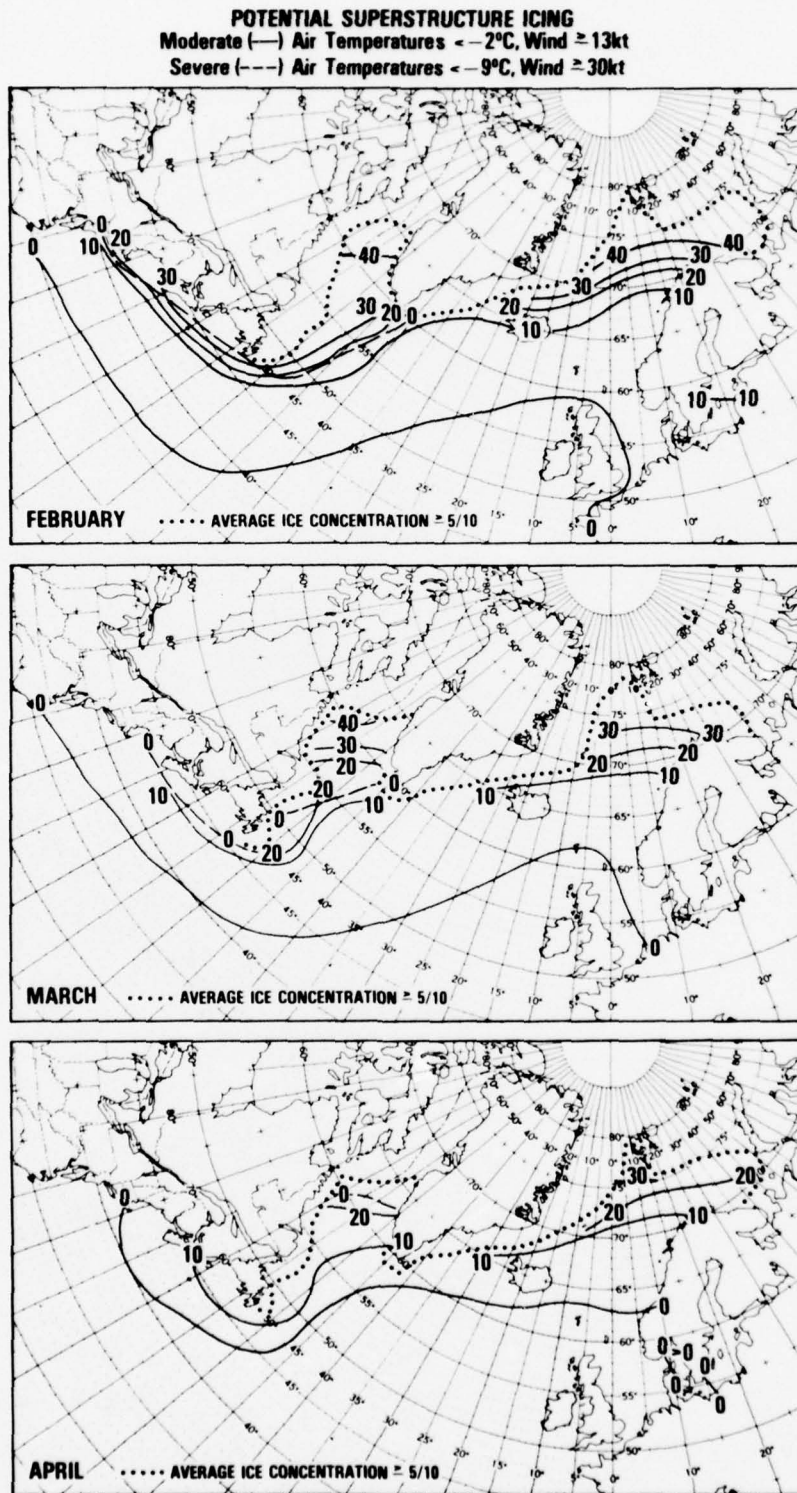
Figure A7. Moderate and severe potential superstructure icing for North Atlantic; February-April (DeAngelis 1974).
