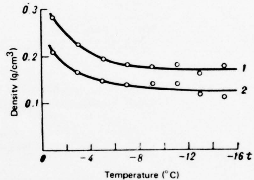
Figure 9. Dependence of density of ice deposit (1 - mixture, 2 - hard rime) on air temperature on meteorological tower at Obninsk, U.S.S.R. (Glukhov 1972).
