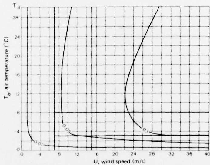
Figure B2. Amount of ice (g/h) which may form on a 1-cm 2 flat surface during ship icing under the following conditions: T_a - T_z = 1^\circ\text{C} , T_a = T_w , S = 0\% , L_z = 80.6 - 94.7 , L_1 = 677 , C_q = 0.50 - 0.46 , C_w = 1.007 (Borisenkov et al. 1971).
