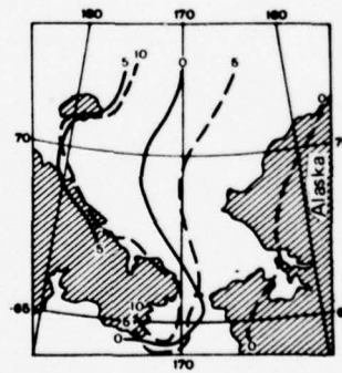
Figure A3. Probability (in percentage) of meteorological conditions conducive to the development of dangerous spray icing (combination of t_a < 0^\circ\text{C} and V >> 15\text{ m/s} ) in September (—) and October (---), from Kolosova (1972).
