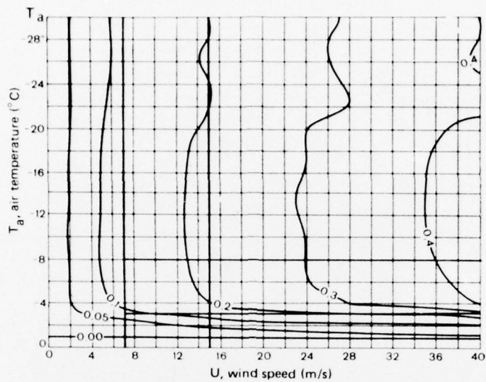
Figure B3. Amount of ice (g/h) which may form on a 1-cm 2 flat surface during ship icing under the following conditions: T_a - T_z = 2^\circ\text{C} , T_a = T_w , S = 15\text{‰} , L_z = 45.0 , L_1 = 646 - 700 , C_q = 0.7 - 18.0 , C_w = 0.98 (Borisenkov et al. 1971).
