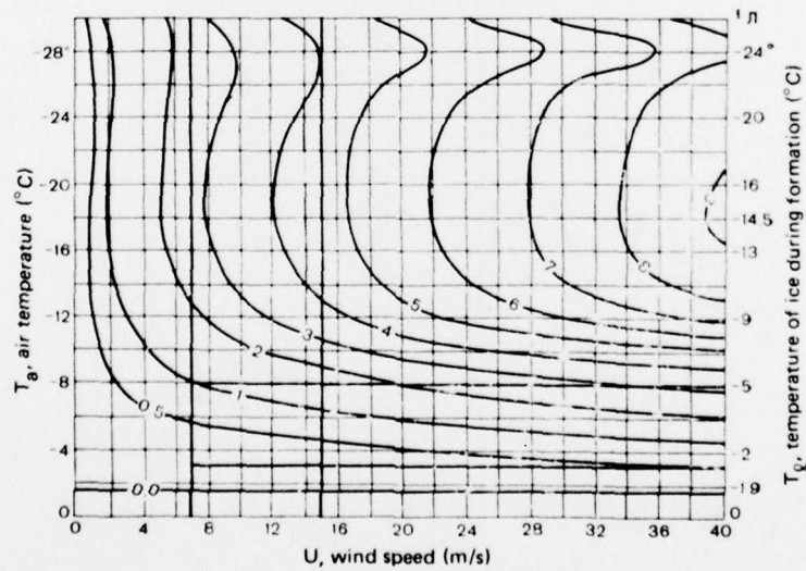
Figure B6. Amount of ice (g/h) which may form on a 1-cm 2 flat surface during ship icing under the following conditions: T_w = 1.7^\circ\text{C} , S = 34\text{ ‰} , L_z = 4.0 , L_i = 601 - 700 , C_q = 1.0 - 36.5 , C_w = 0.96 (Borisenkov et al. 1971).
