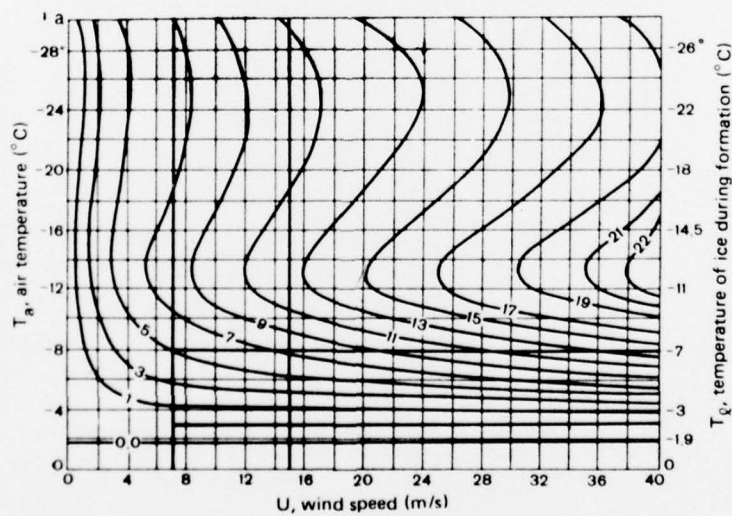
Figure B4. Amount of ice (g/h) which may form on a 1-cm 2 surface of a 1-cm-diam cylinder during ship icing under the following conditions: T_w = -1.7^\circ\text{C} , S = 34\text{‰} , L_z = 4.0 , L_1 = 601 - 700 , C_q = 0.6 - 36.5 , C_w = 0.96 (Borisenkov et al. 1971).
