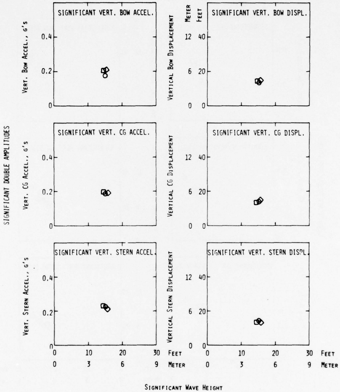
Figure 59 - Significant Double Amplitudes of Vertical Accelerations and Vertical Motions in Random Head Seas for SWATH 6 - 28 Knots
