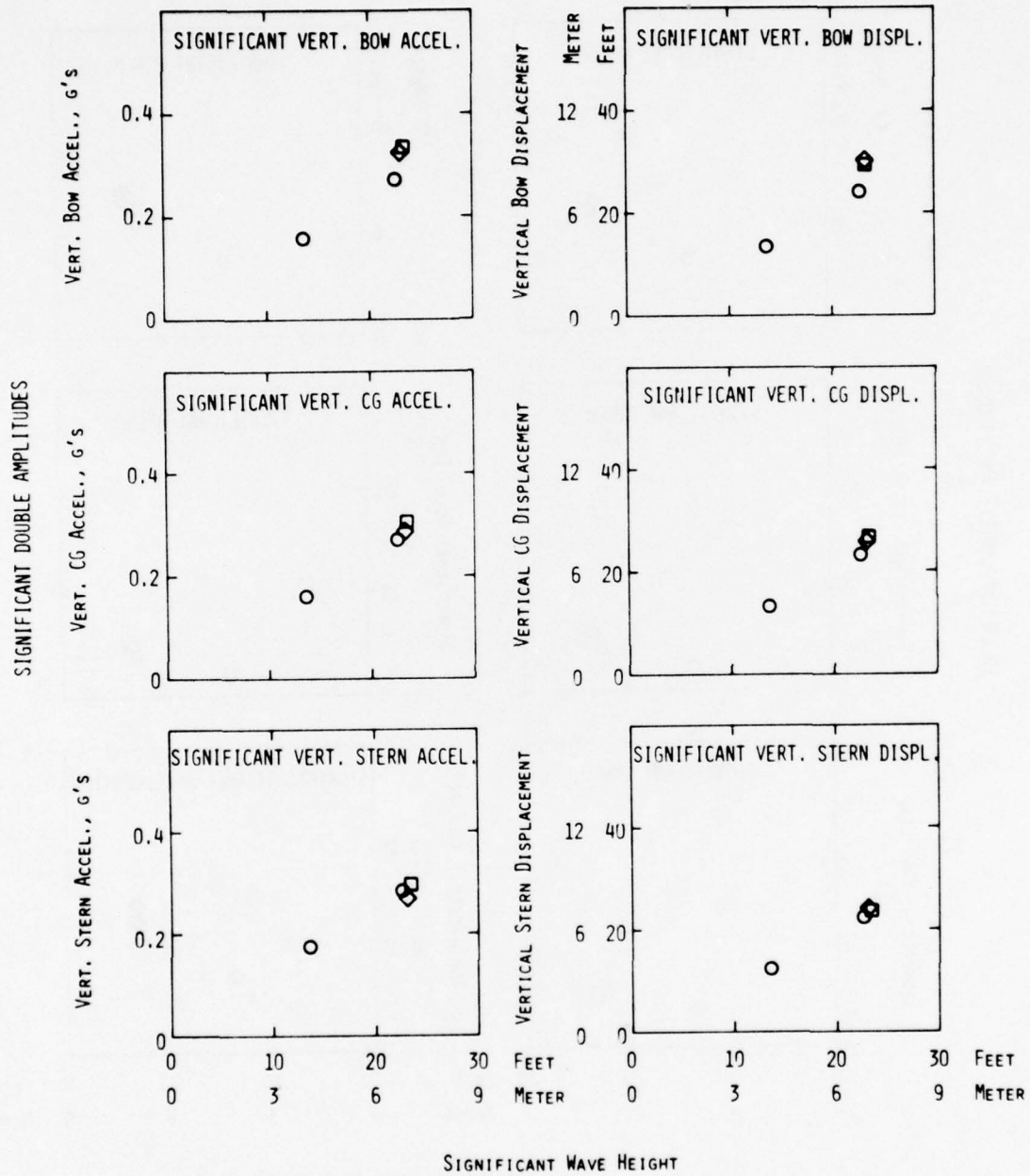
Figure 72 - Significant Double Amplitudes of Vertical Accelerations and Vertical Motions in Random Bow Quartering Seas for SWATH 6 - 20 Knots
