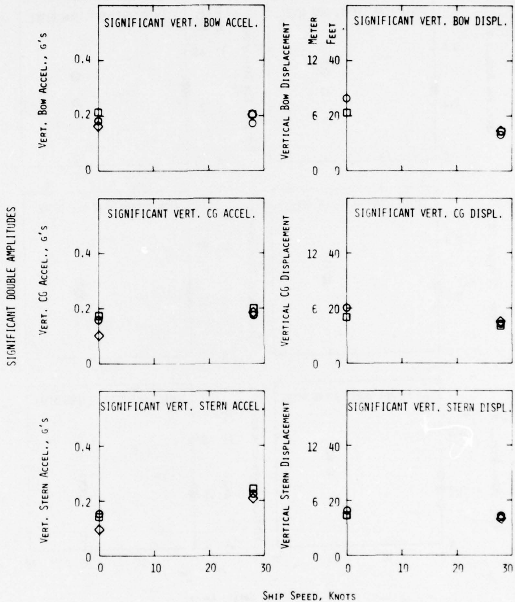
Figure 60 - Significant Double Amplitudes of Vertical Accelerations and Vertical Motions in Head Sea State 6 for SWATH 6
