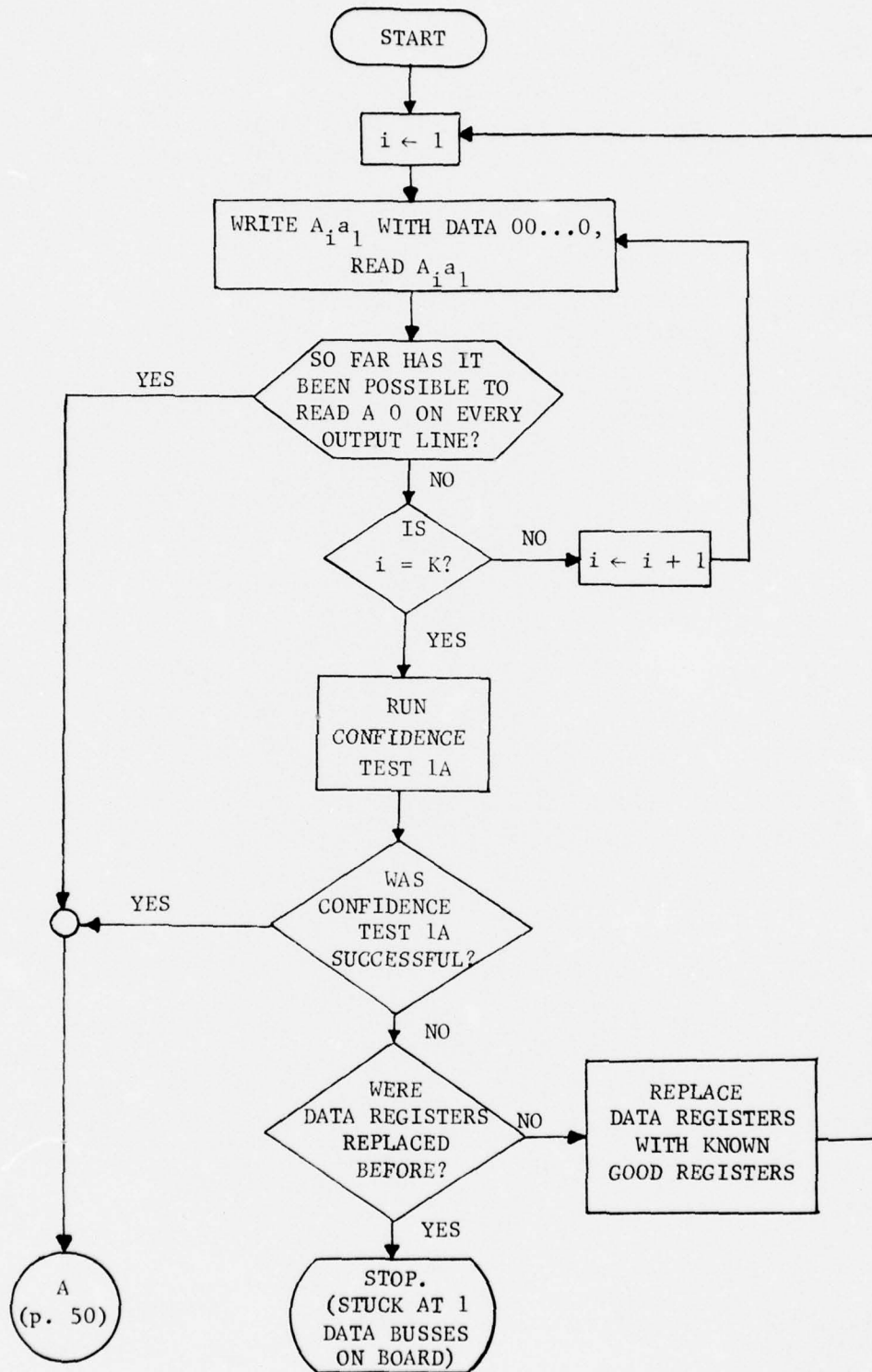
Figure 4.2(a). Test procedure for testing data buses.
