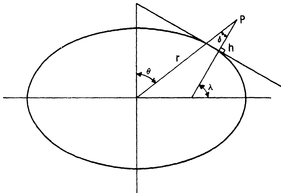
Figure 2-2. Exaggerated ellipse illustrating the geocentric coordinates r , \theta , and the geodetic latitude, \lambda , and altitude, h , of a point P . ( \delta is the rotational angle between the geocentric and geodetic vectors (B_\theta, B_r) and (X, Z) , respectively.)
