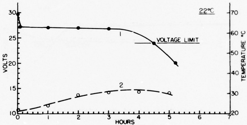
Fig. 14: Discharge at 22^{\circ}\text{C} and a Constant Current of 3.0A of Battery No. 36. 1. Voltage 2. Temperature
