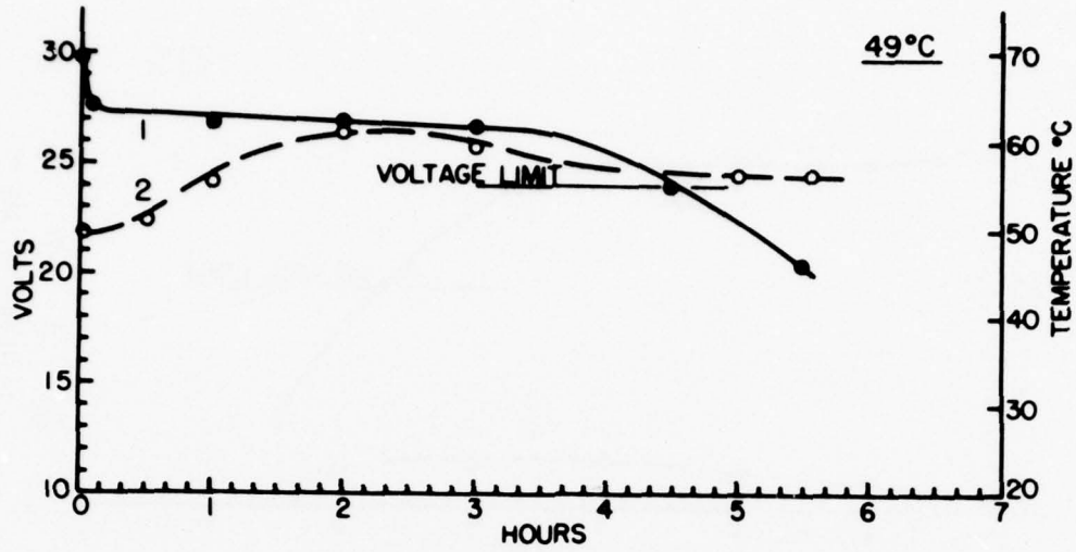
Fig. 15: Discharge at 49°C of Battery No. 47. 1. Voltage 2. Temperature
