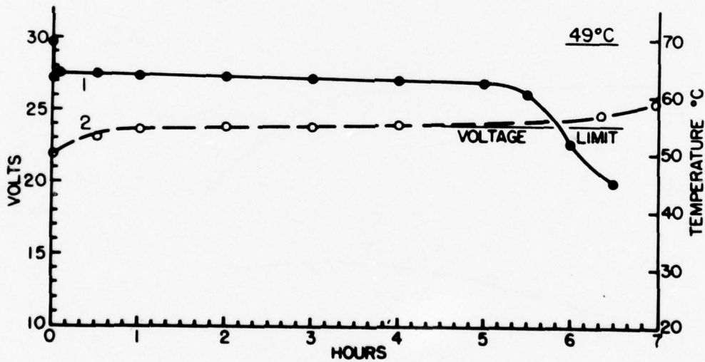
Fig. 16: Discharge at 49°C of Battery No. 49. 1. Voltage 2. Temperature
