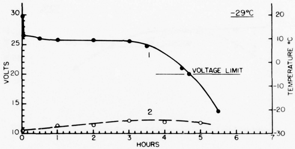
Fig. 13: Discharge at -29^{\circ}\text{C} of Battery No. 45. 1. Voltage 2. Temperature
