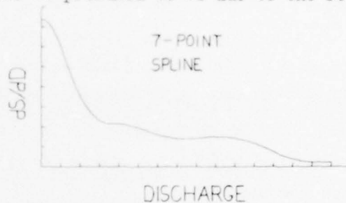
Fig. 8. Derivative for 7-point spline fit
