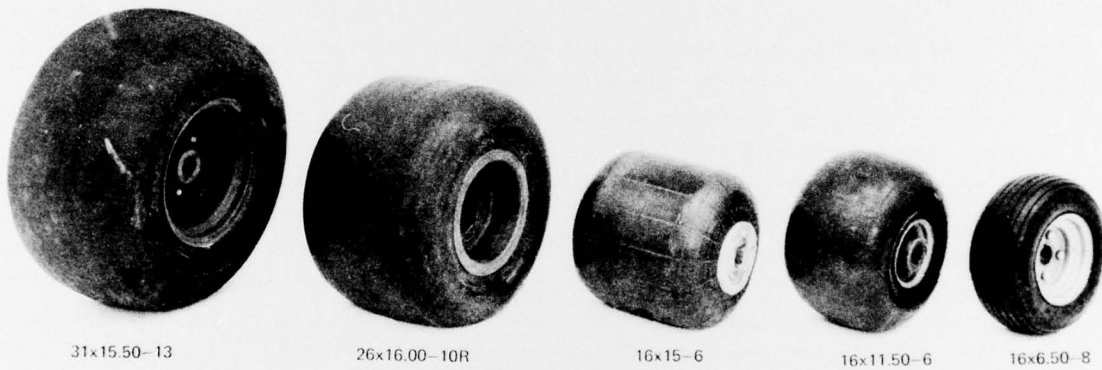
Fig. 3. Rectangular-cross-section tires
