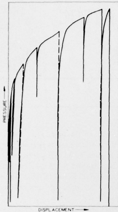
Fig. 2. Typical pressure-displacement curve, horizontal jacking test
