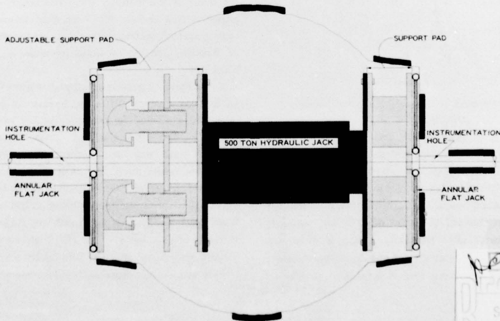
Fig. 1. Horizontal jacking equipment. DISTRIBUTION STATEMENT A Approved for public release; Distribution Unlimited
