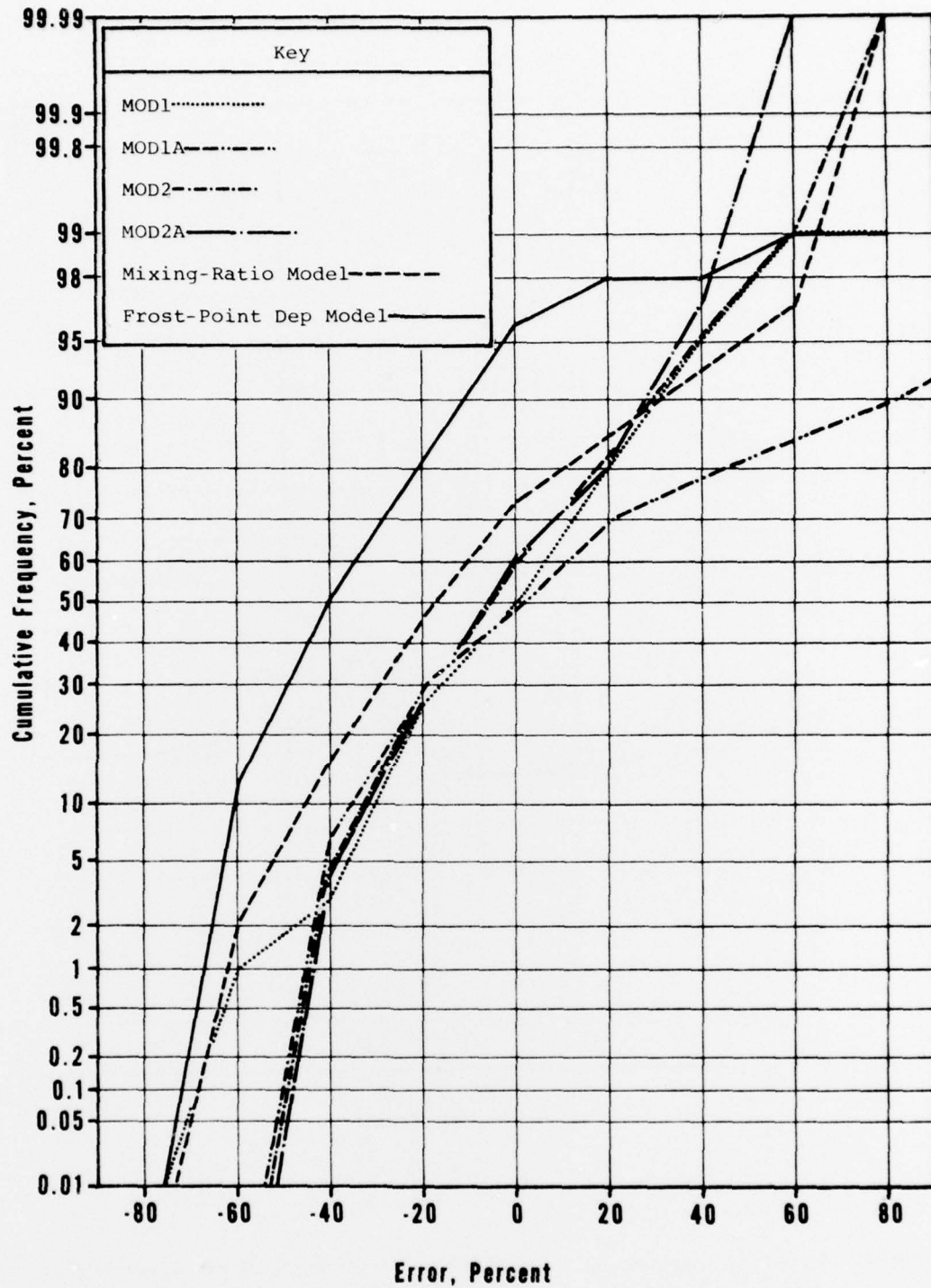
Figure 3. Cumulative Frequency of Error in Precipitable Water in Column from 10 km Above Tropopause to the T = -40^{\circ}\text{C} Level - Dependent Data
