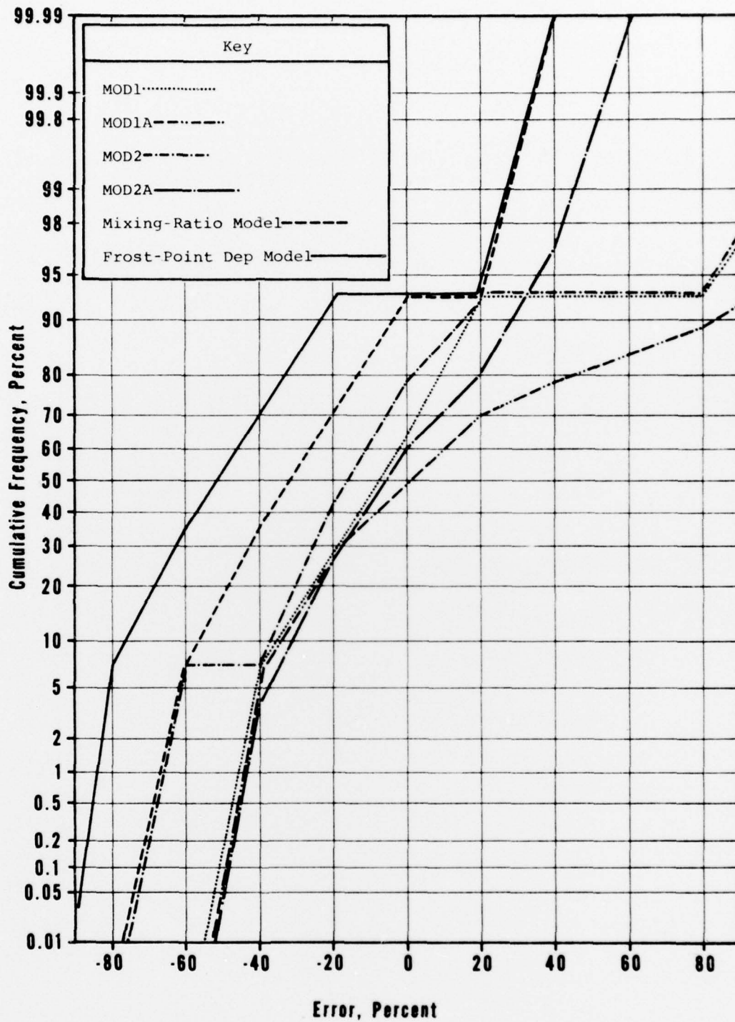
Figure 4. Cumulative Frequency of Error in Precipitable Water in Column from 10 km Above Tropopause to the T = -40^{\circ}\text{C} Level - Independent Data
