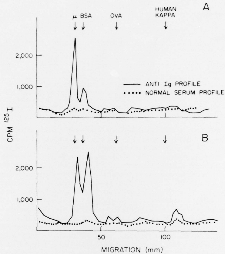
FIG. 4. SDS-polyacrylamide gel electropherogram of ^{125}\text{I} -labeled membrane immunoglobulin specifically precipitated from (CBA/N \times DBA/2 \delta ) F_1 female spleen cells pretreated with (A) absorbed C57BL/6 anti-DBA/2 serum + C. (B) NMS + C.
