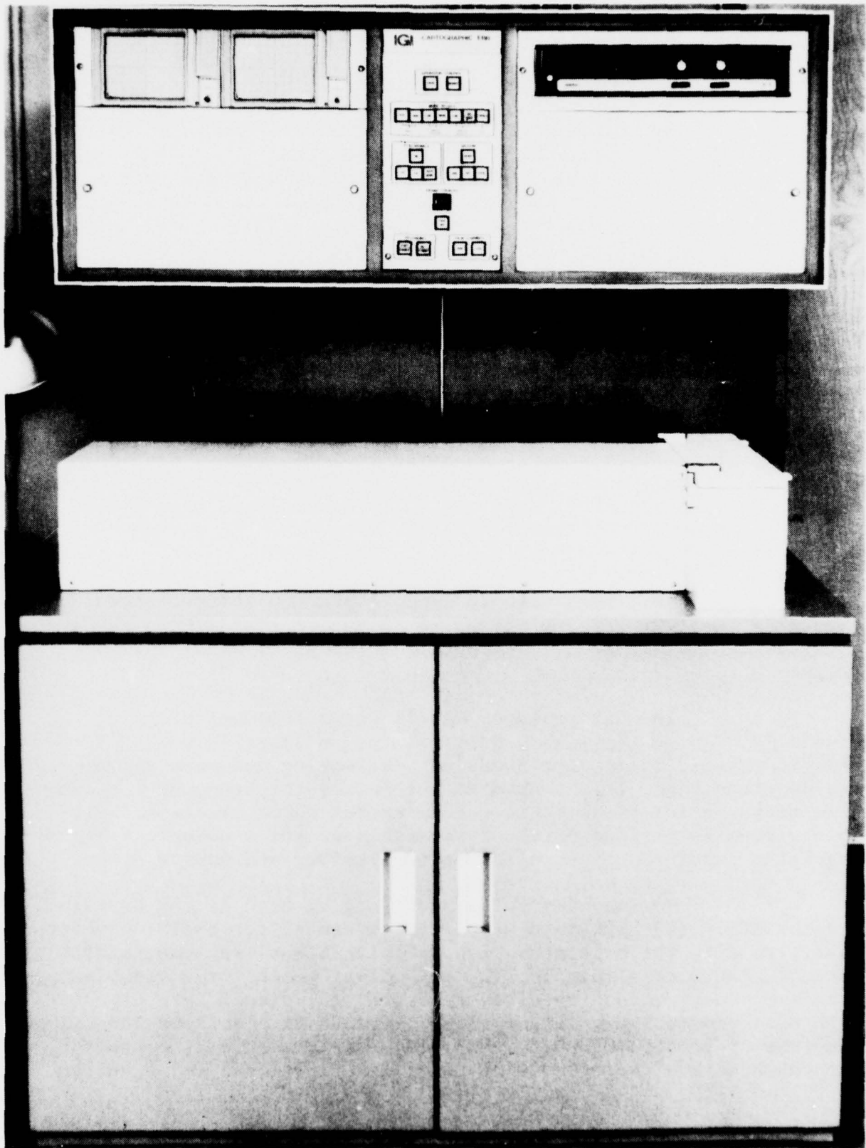
Figure 18. Image Graphics, Inc. - EBR 2000
