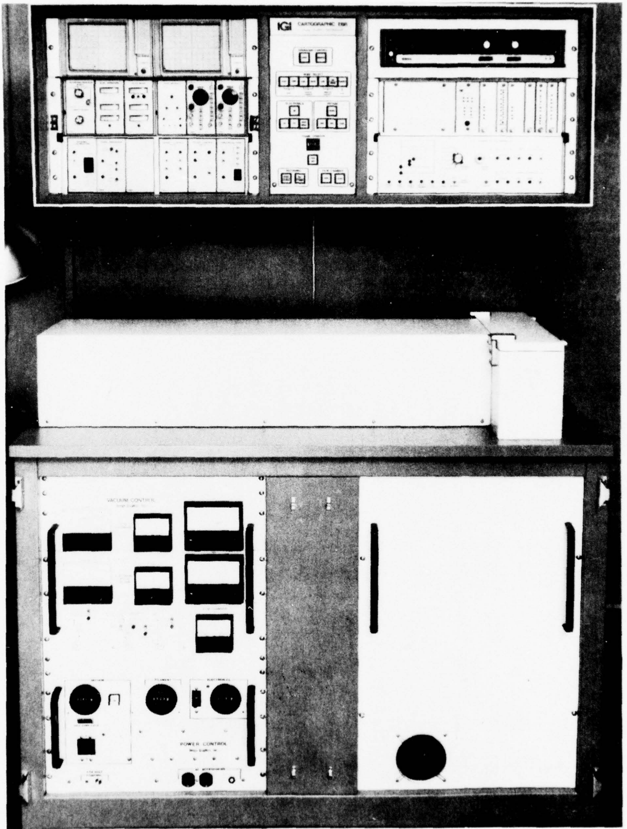
Figure 20. Cartographic EBR - Front View - Doors Removed 41
