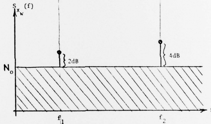
Figure 3 (b) SLE Noise Prewhitener Output Power Spectrum (Idealized)
