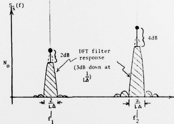
FIGURE 3. SLE Example of a Two Line Component Signal in Colored Noise.
