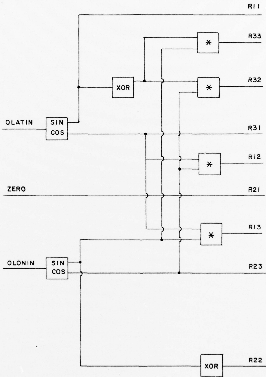
FIGURE 16 - INITIALIZATION OF POSITION MATRIX R
