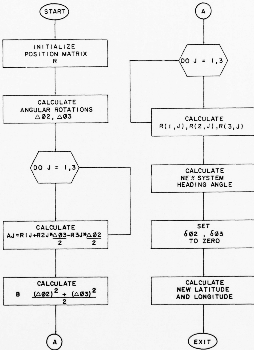
FIGURE 15 - NAVIGATION PROCESSING FLOWCHART
