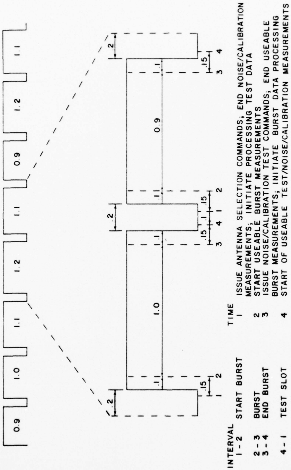
FIGURE 11 - BURST FILTER TIME INTERVAL
