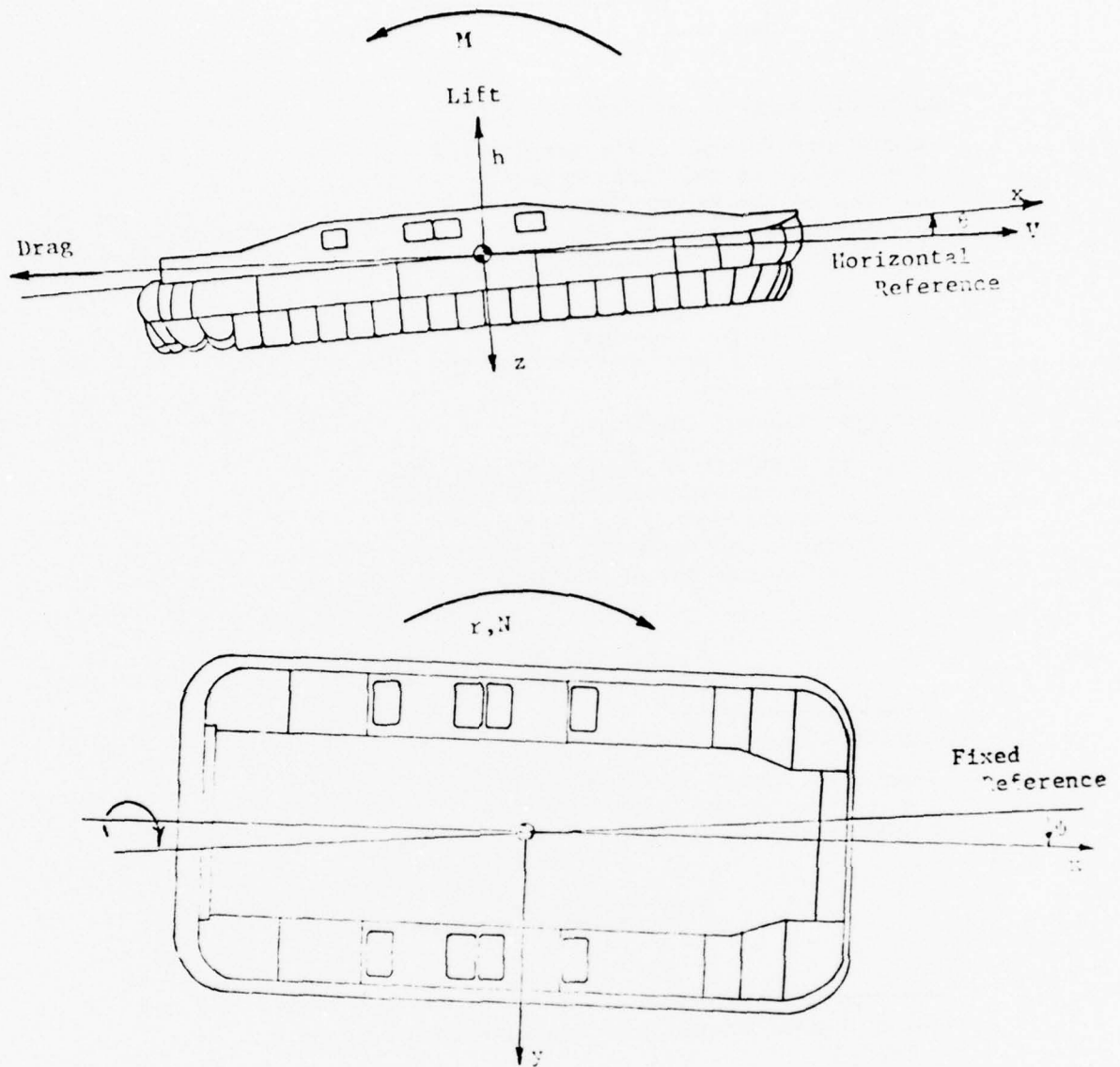
Figure 1 - Schematic Indicating Positive Directions of Measured Quantities
